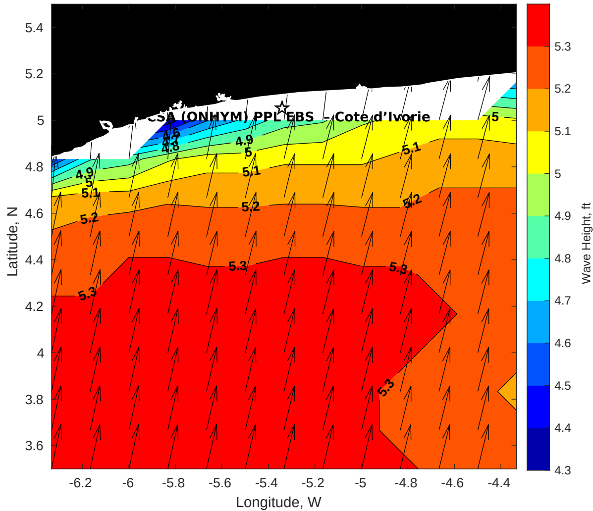
Wave Height (ft) for CSA (ONHYM) PPL EBS - Cote d'Ivoire at 18-Jul-2025 09:00:00
