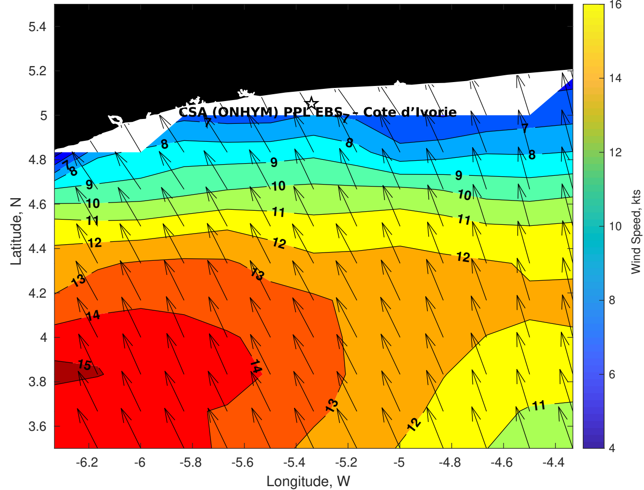
Winds (kts) for CSA (ONHYM) PPL EBS - Cote d'Ivoire at 18-Jul-2025 09:00:00
