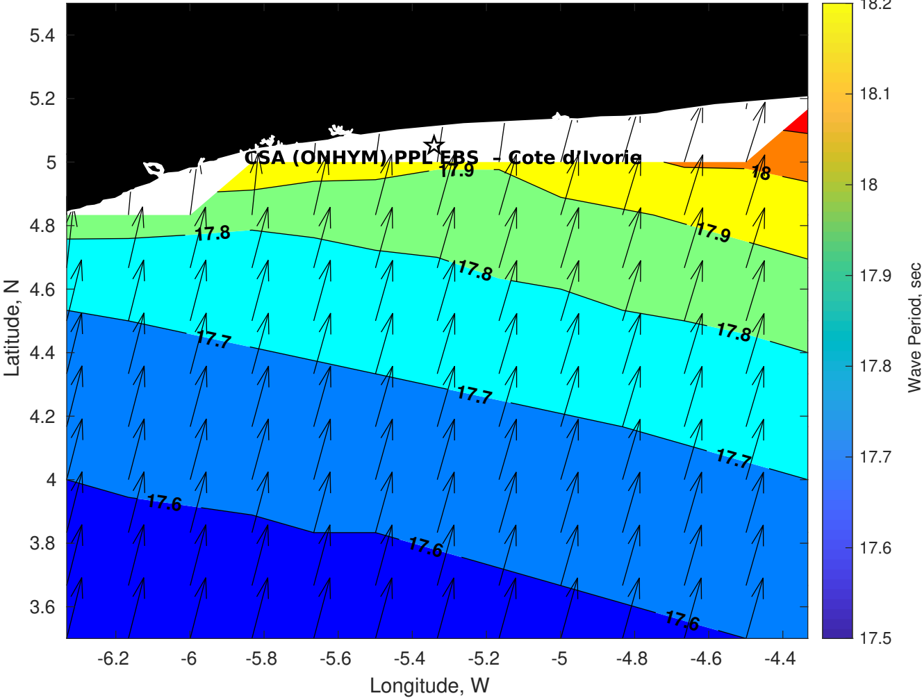
Wave Period (sec) for CSA (ONHYM) PPL EBS - Cote d'Ivoire at 18-Jul-2025 09:00:00
