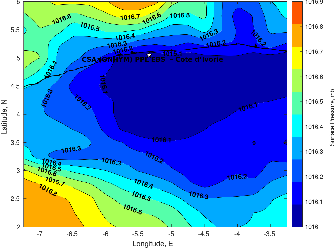
Surface Pressure (mb) for CSA (ONHYM) PPL EBS - Cote d'Ivoire at 18-Jul-2025 00:00:00
