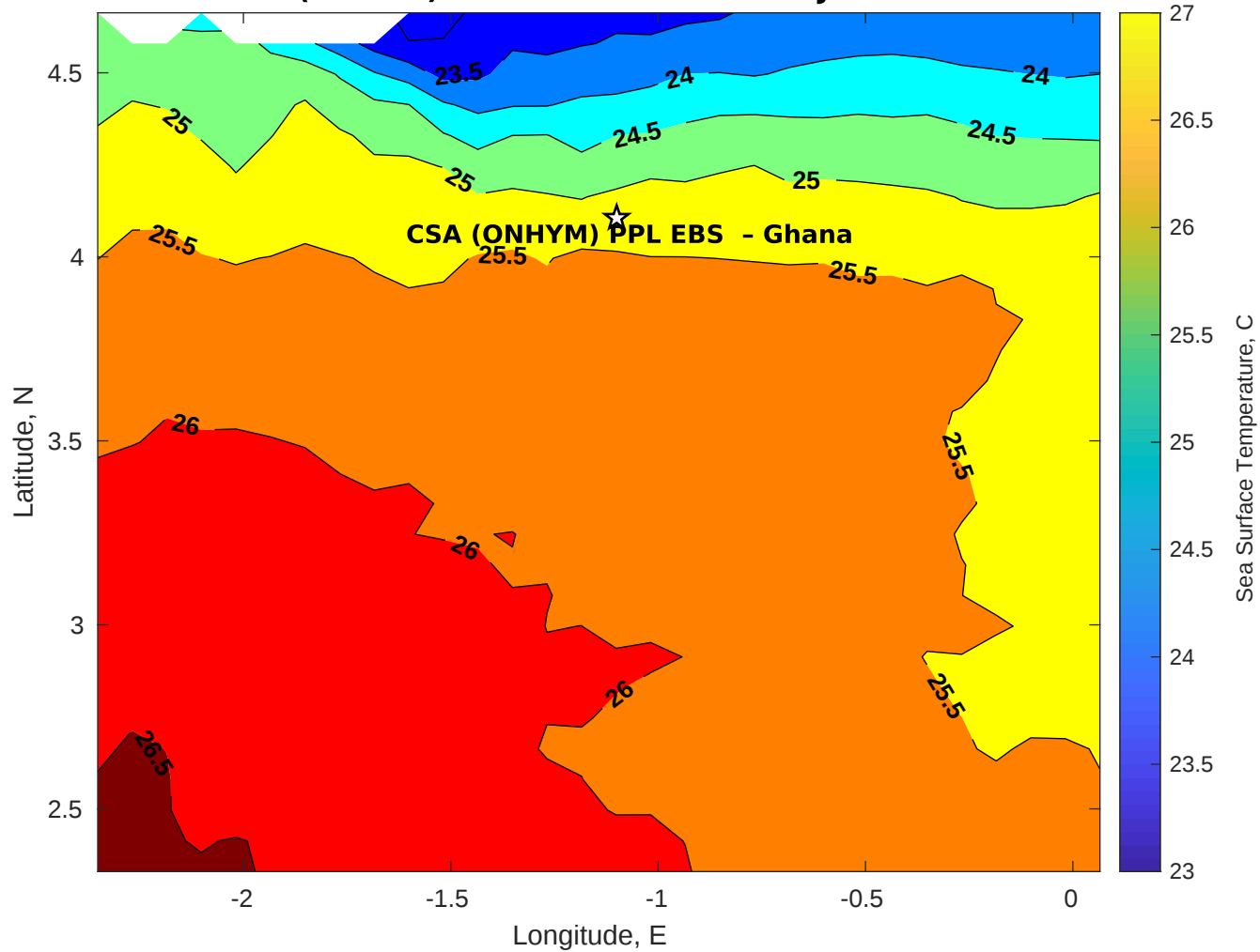
SST for CSA (ONHYM) PPL EBS - Ghana at 17-Jul-2025 00:00:00
