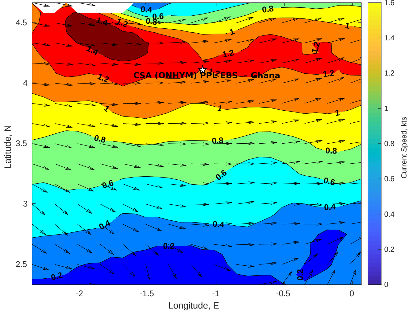
Surface Currents for CSA (ONHYM) PPL EBS - Ghana at 17-Jul-2025 00:00:00
