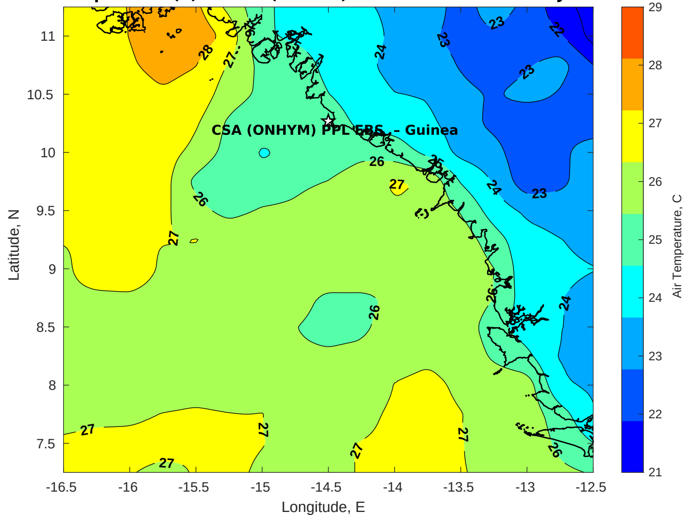
Air Temperature (C) for CSA (ONHYM) PPL EBS - Guinea at 18-Jul-2025
