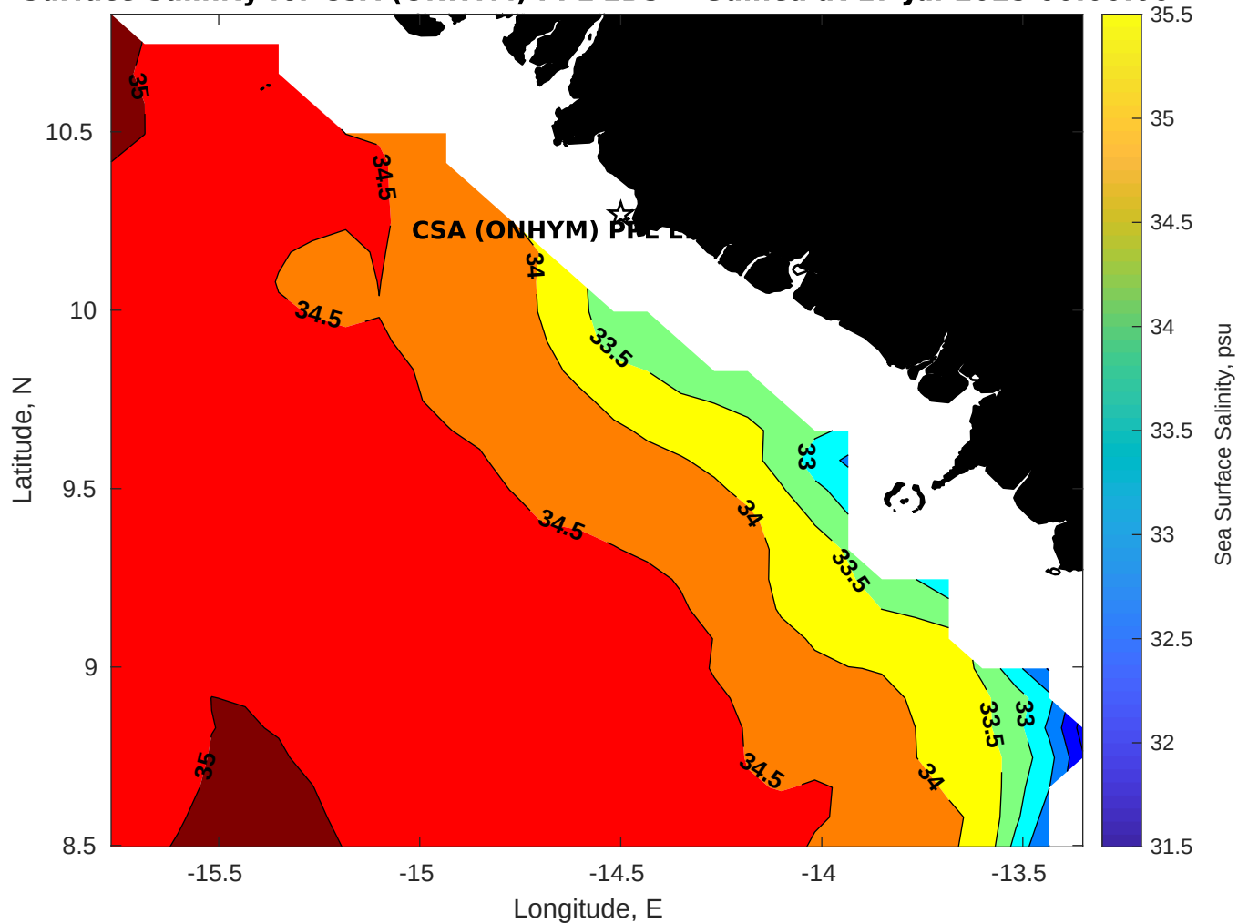
Surface Salinity for CSA (ONHYM) PPL EBS - Guinea at 17-Jul-2025 00:00:00
