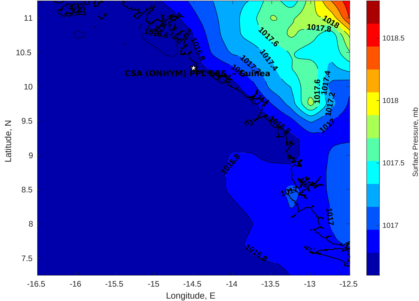
Surface Pressure (mb) for CSA (ONHYM) PPL EBS - Guinea at 20-Jul-2025 00:00:00
