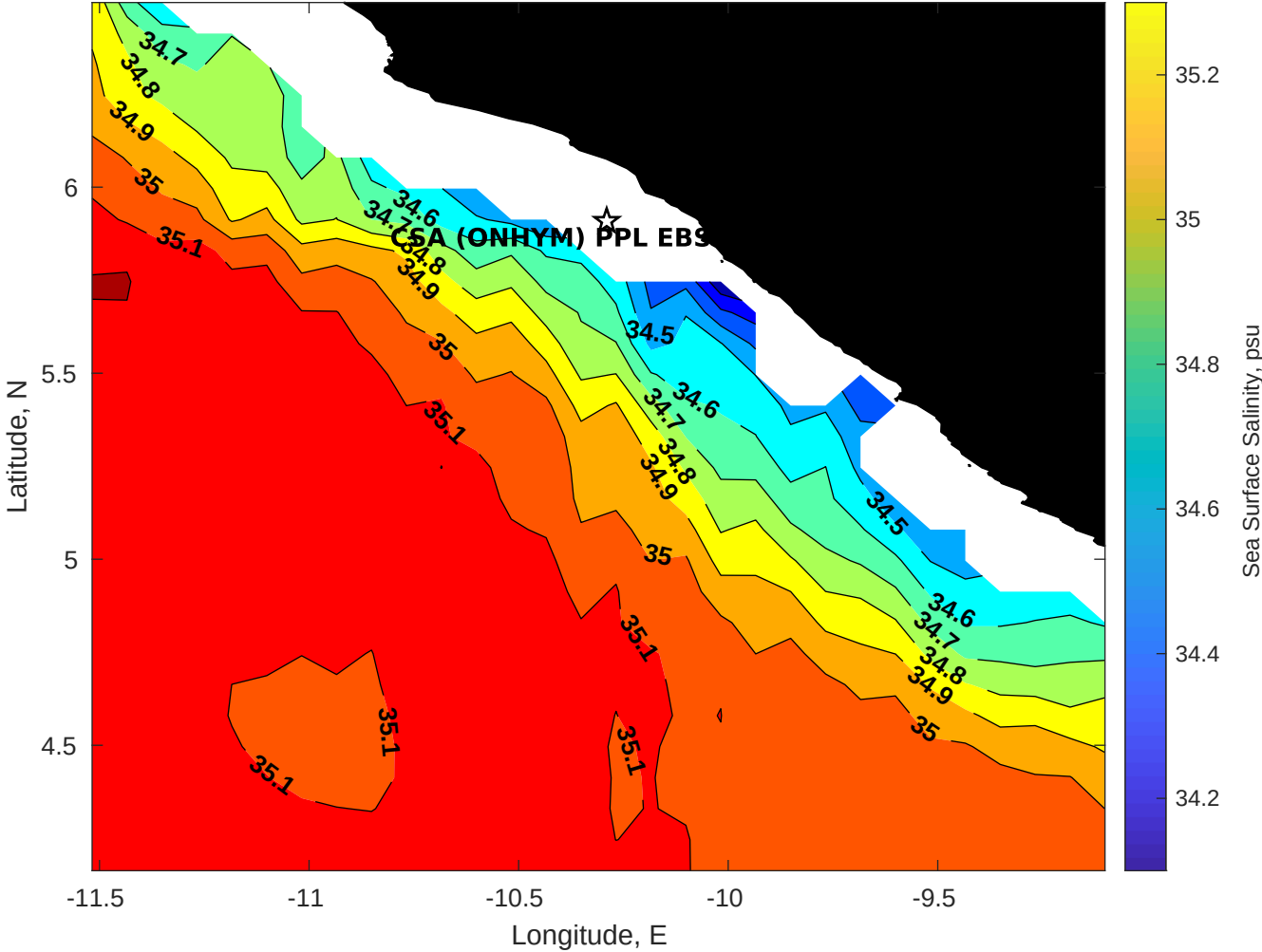
Surface Salinity for CSA (ONHYM) PPL EBS - Liberia at 17-Jul-2025 00:00:00
