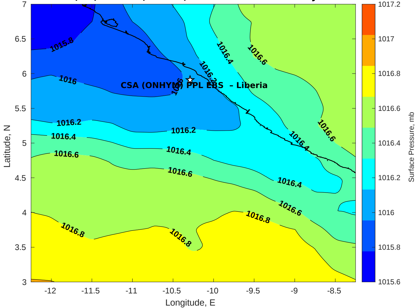
Surface Pressure (mb) for CSA (ONHYM) PPL EBS - Liberia at 18-Jul-2025 00:00:00
