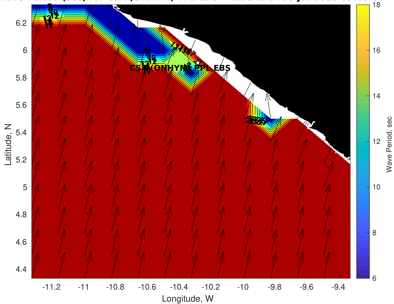
Wave Period (sec) for CSA (ONHYM) PPL EBS - Liberia at 18-Jul-2025 09:00:00
