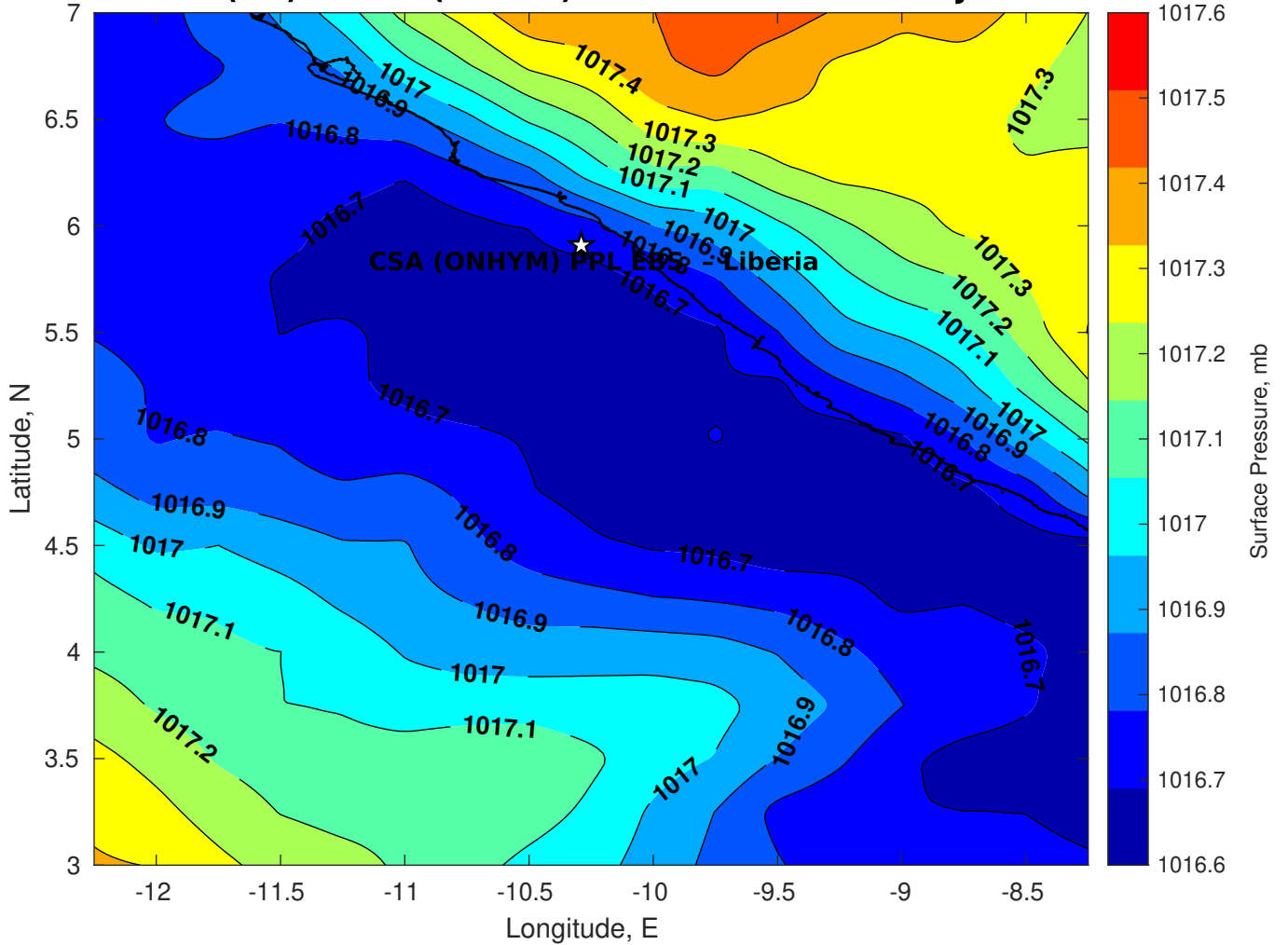
Surface Pressure (mb) for CSA (ONHYM) PPL EBS - Liberia at 20-Jul-2025 00:00:00
