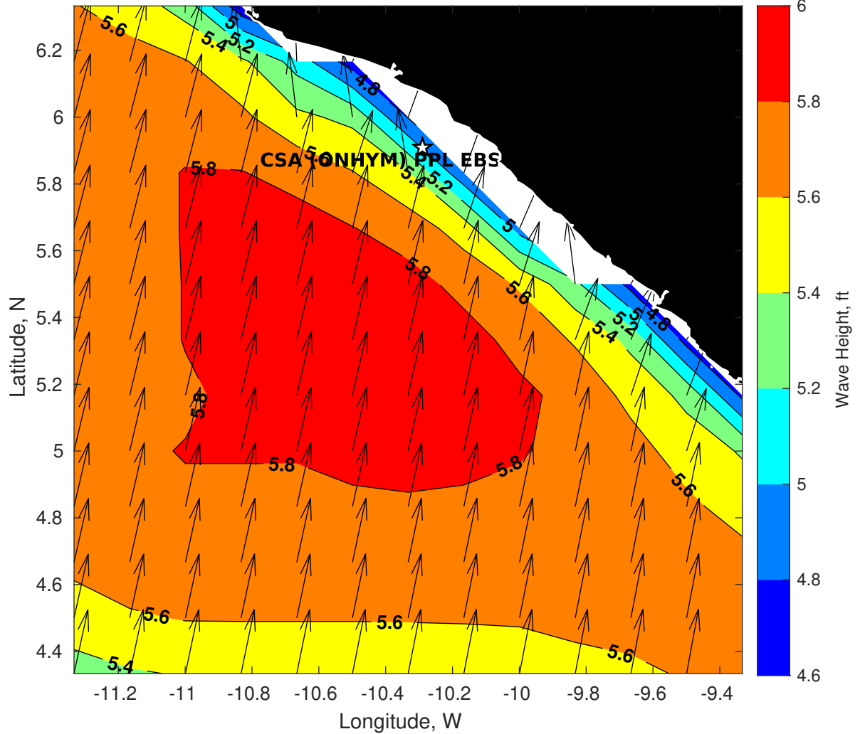
Wave Height (ft) for CSA (ONHYM) PPL EBS - Liberia at 18-Jul-2025 09:00:00
