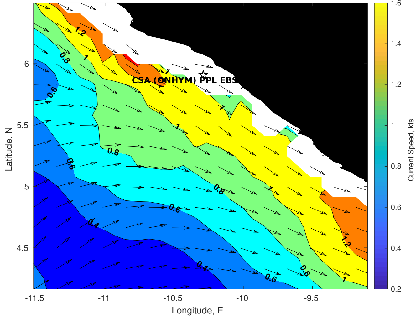
Surface Currents for CSA (ONHYM) PPL EBS - Liberia at 17-Jul-2025 00:00:00
