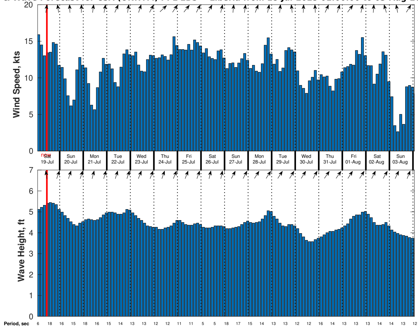
Wind & Wave Forecast for CSA (ONHYM) PPL EBS - Liberia from 18-Jul-2025 01:00:00 to 03-Aug-2025 01:00:00
