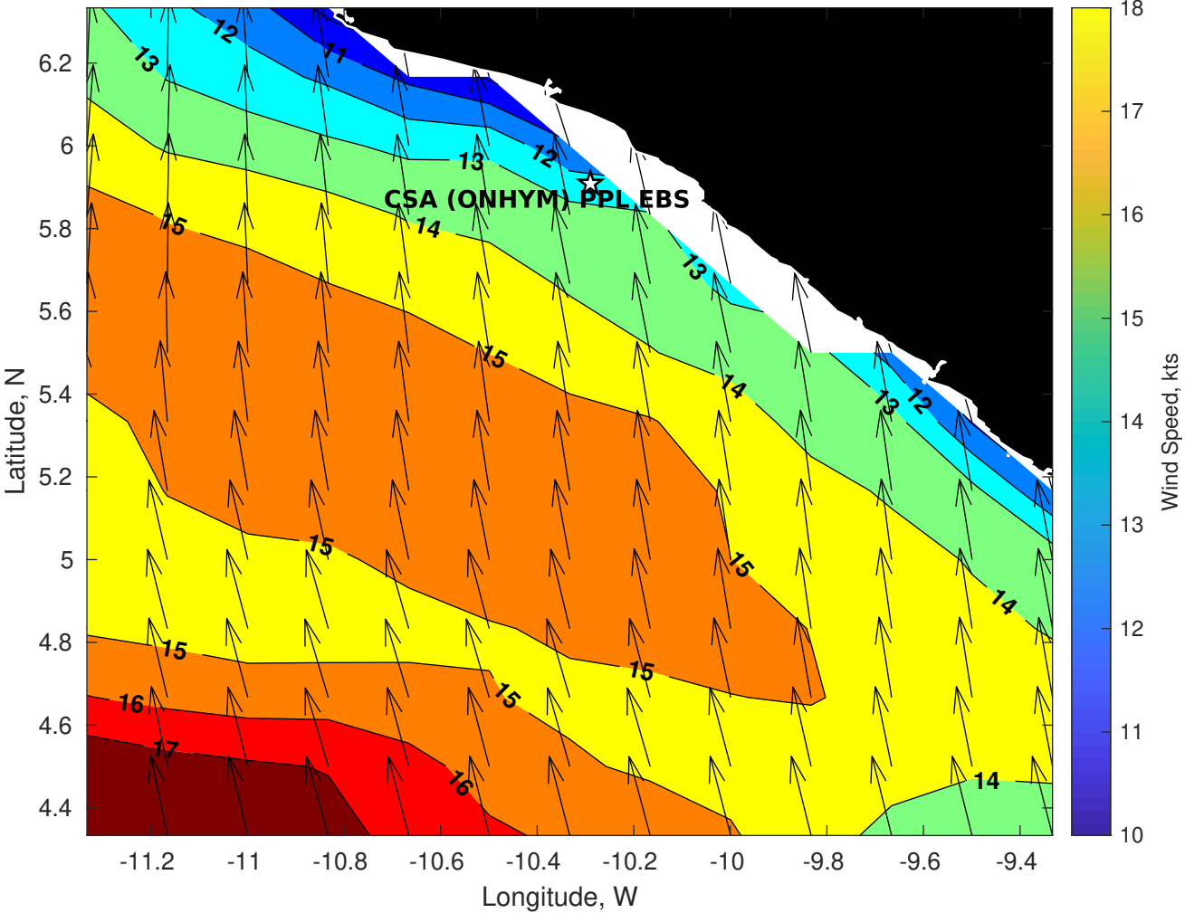
Winds (kts) for CSA (ONHYM) PPL EBS - Liberia at 18-Jul-2025 09:00:00
