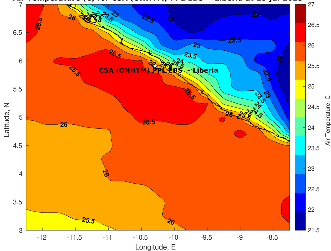
Air Temperature (C) for CSA (ONHYM) PPL EBS - Liberia at 18-Jul-2025
