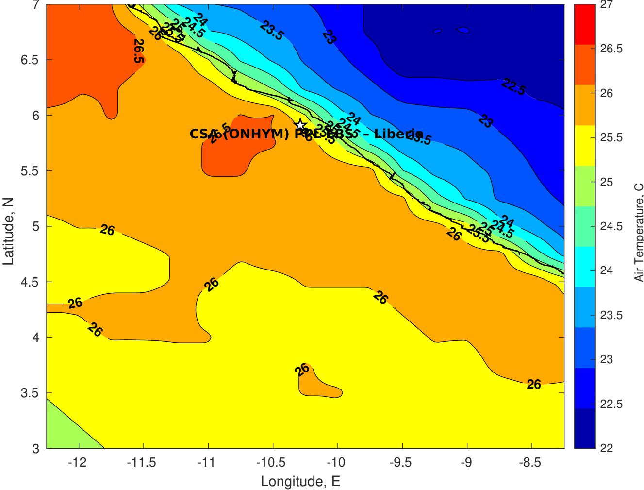
Air Temperature (C) for CSA (ONHYM) PPL EBS - Liberia at 18-Jul-2025
