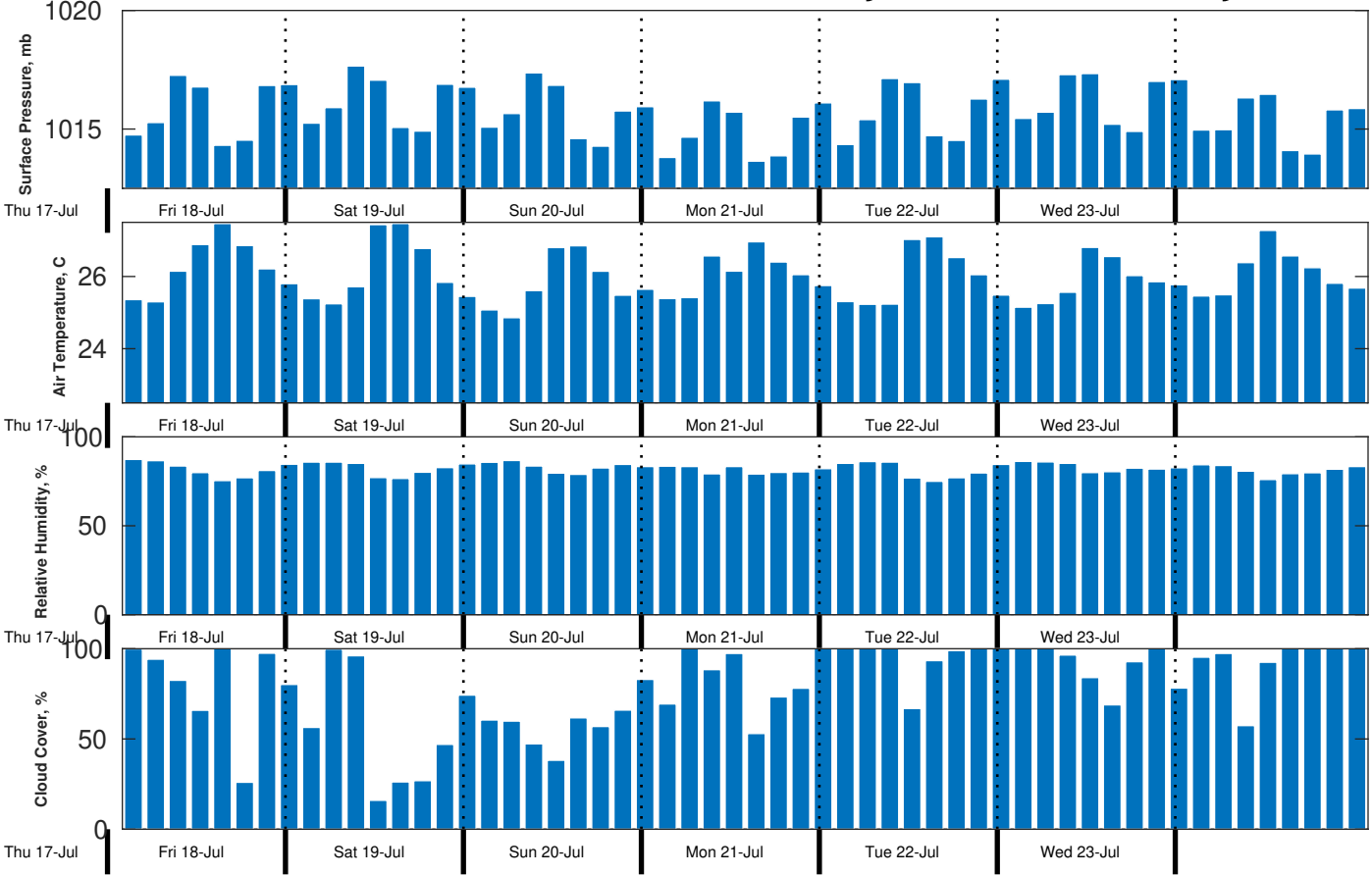
Met Forecast for CSA (ONHYM) PPL EBS - Liberia from 18-Jul-2025 00:00:00 to 25-Jul-2025 00:00:00
