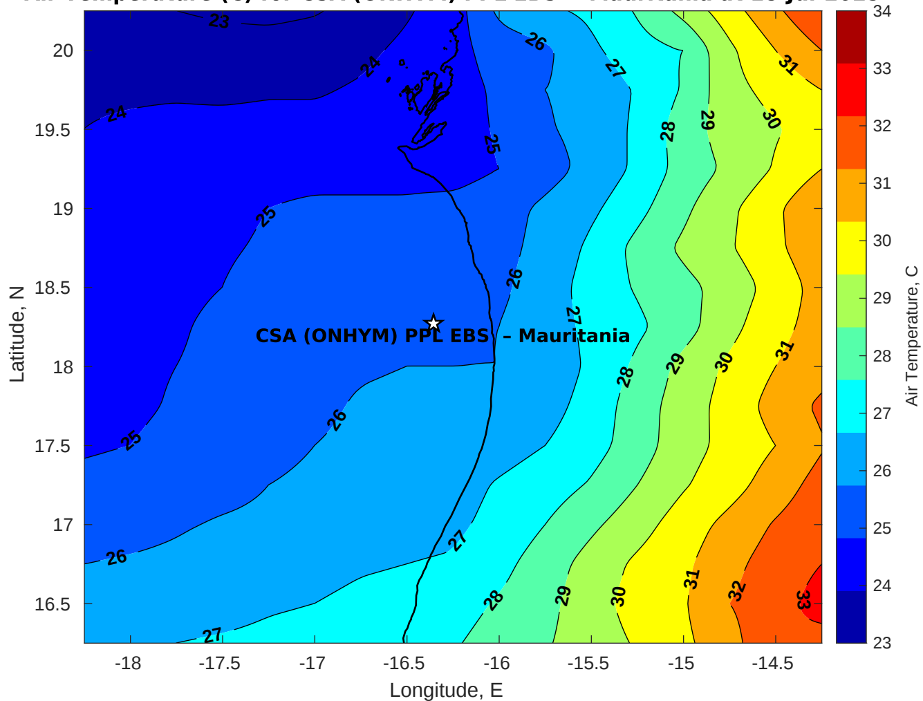
Air Temperature (C) for CSA (ONHYM) PPL EBS - Mauritania at 18-Jul-2025
