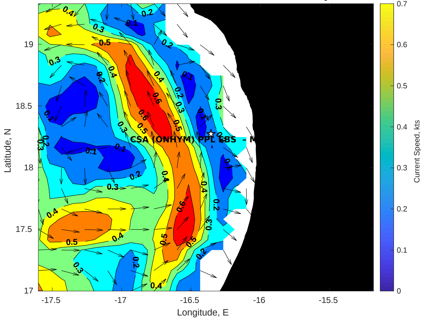
Surface Currents for CSA (ONHYM) PPL EBS - Mauritania at 17-Jul-2025 00:00:00
