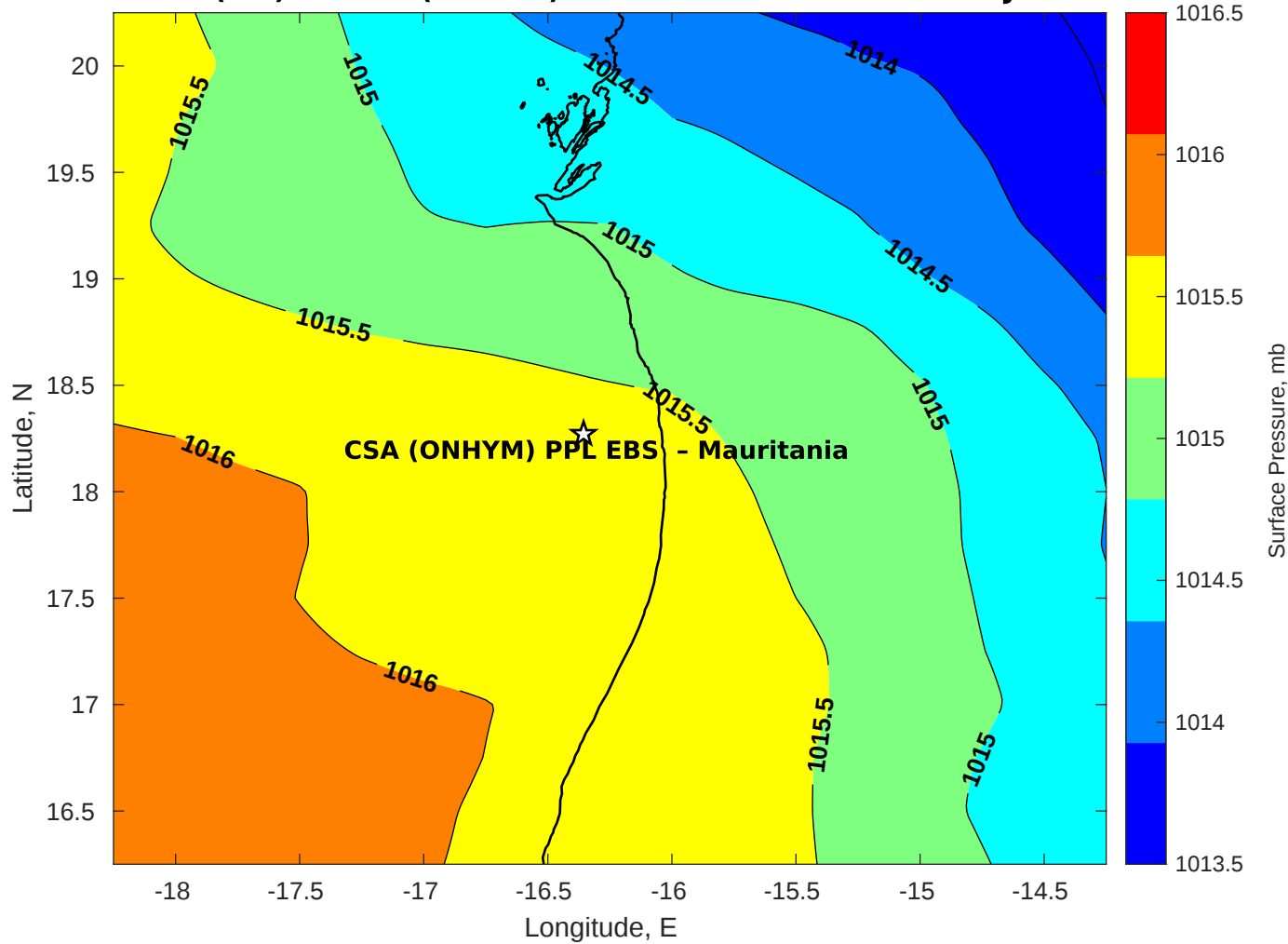
Surface Pressure (mb) for CSA (ONHYM) PPL EBS - Mauritania at 20-Jul-2025 00:00:00
