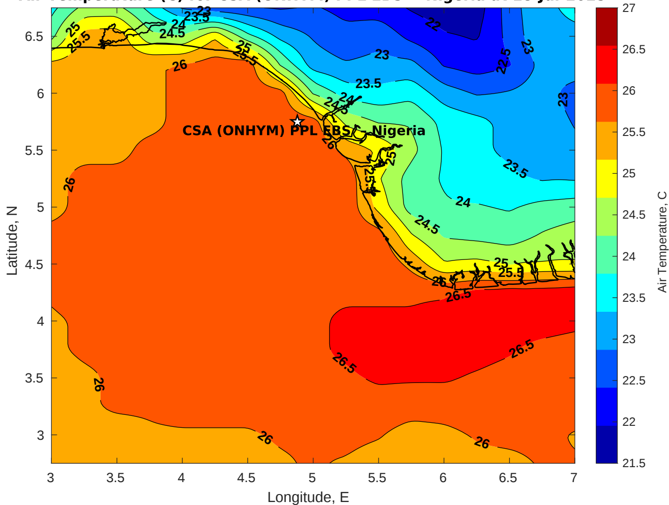
Air Temperature (C) for CSA (ONHYM) PPL EBS - Nigeria at 18-Jul-2025
