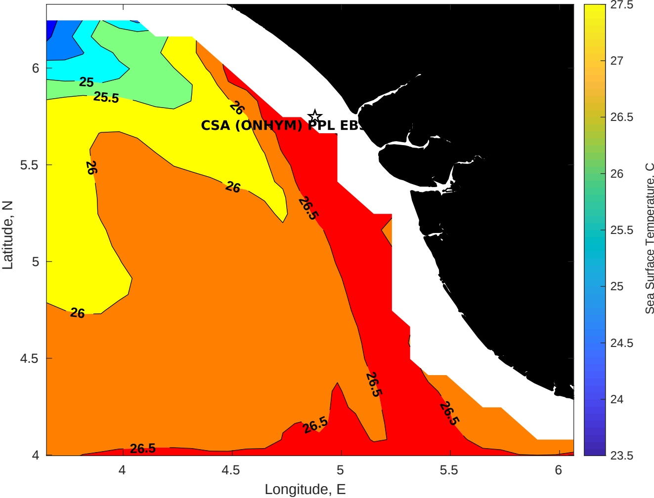
SST for CSA (ONHYM) PPL EBS - Nigeria at 17-Jul-2025 00:00:00
