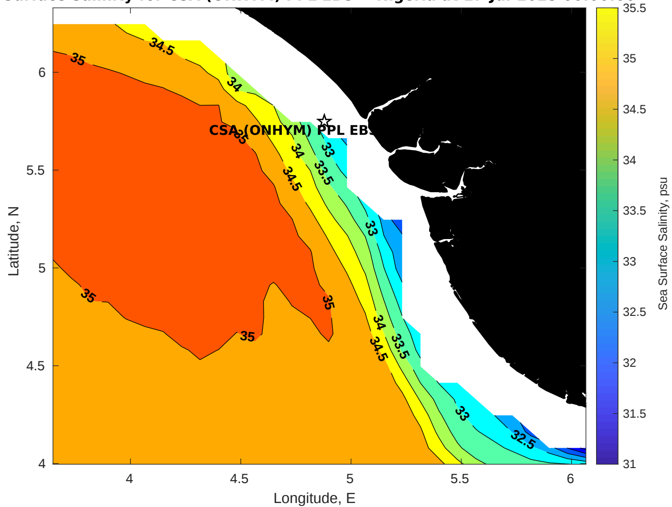
Surface Salinity for CSA (ONHYM) PPL EBS - Nigeria at 17-Jul-2025 00:00:00
