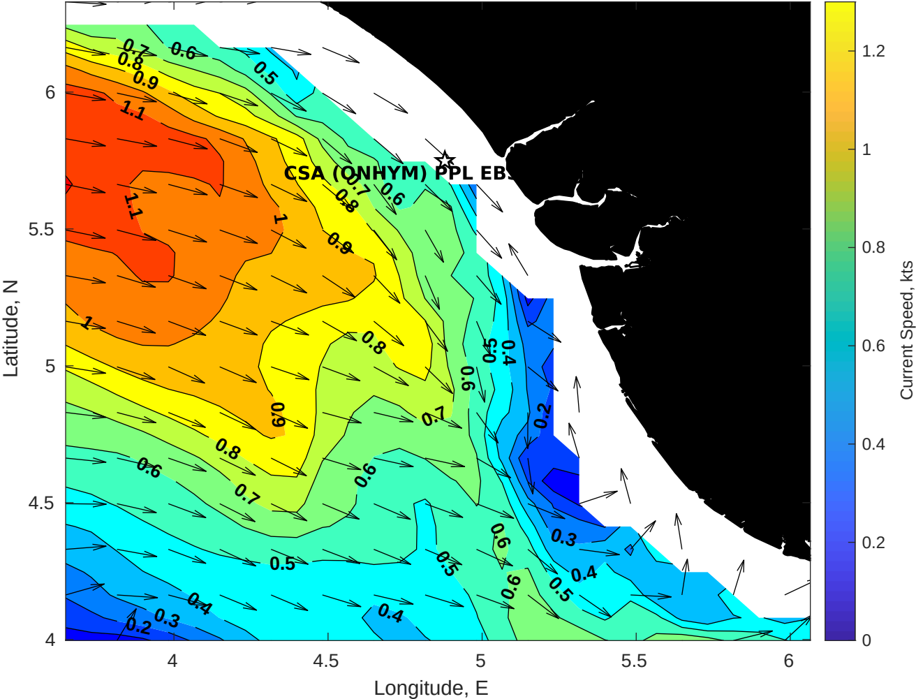
Surface Currents for CSA (ONHYM) PPL EBS - Nigeria at 17-Jul-2025 00:00:00
