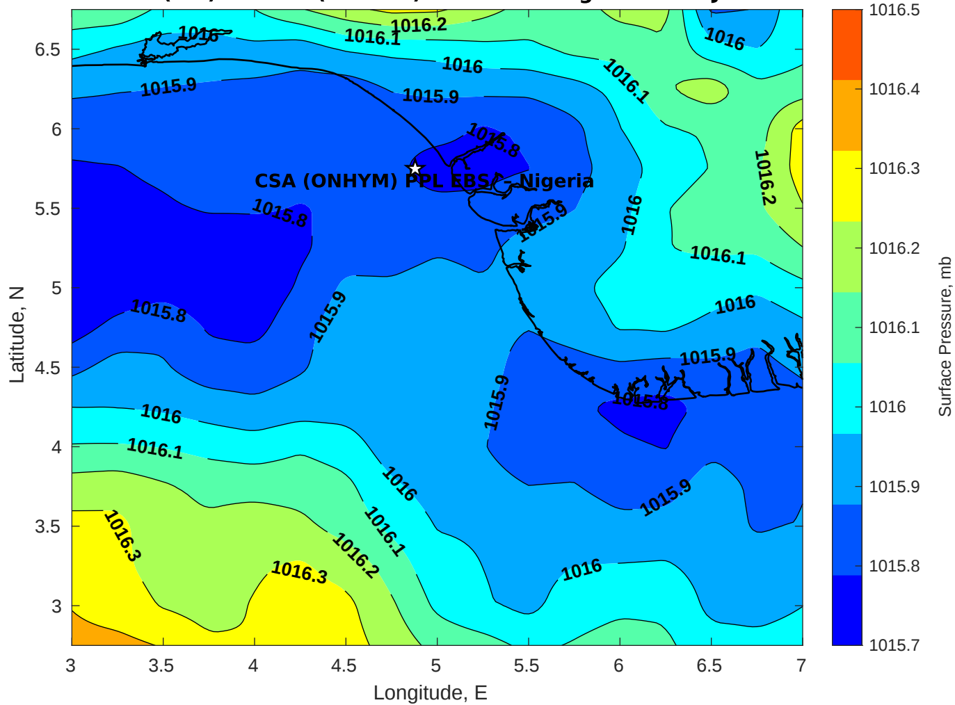
Surface Pressure (mb) for CSA (ONHYM) PPL EBS - Nigeria at 18-Jul-2025 00:00:00
