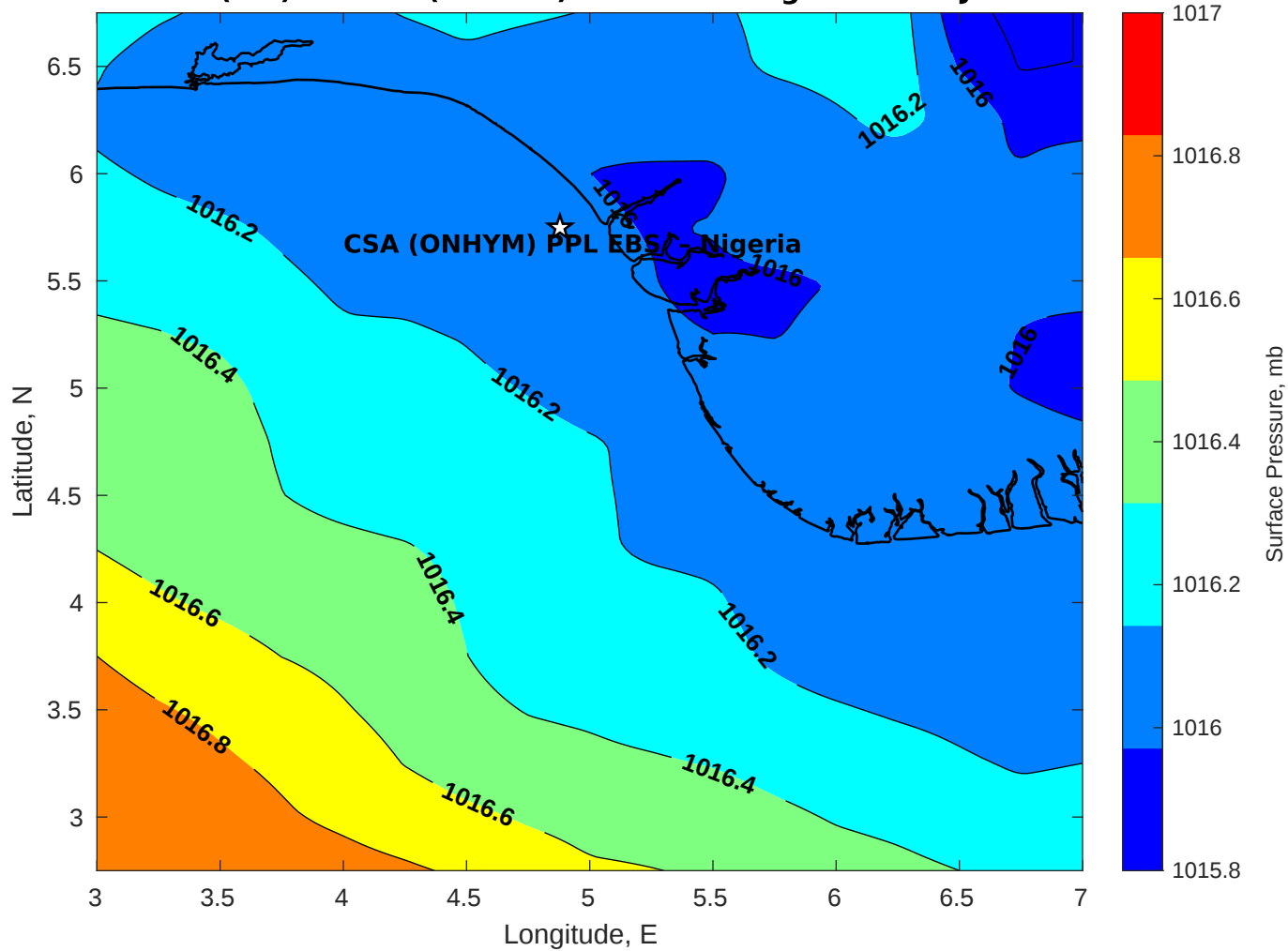
Surface Pressure (mb) for CSA (ONHYM) PPL EBS - Nigeria at 19-Jul-2025 00:00:00
