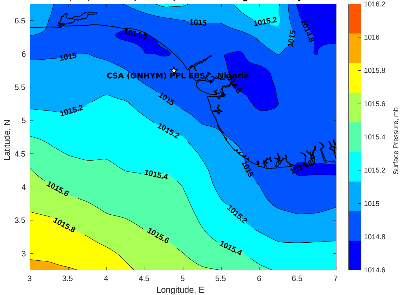
Surface Pressure (mb) for CSA (ONHYM) PPL EBS - Nigeria at 20-Jul-2025 00:00:00
