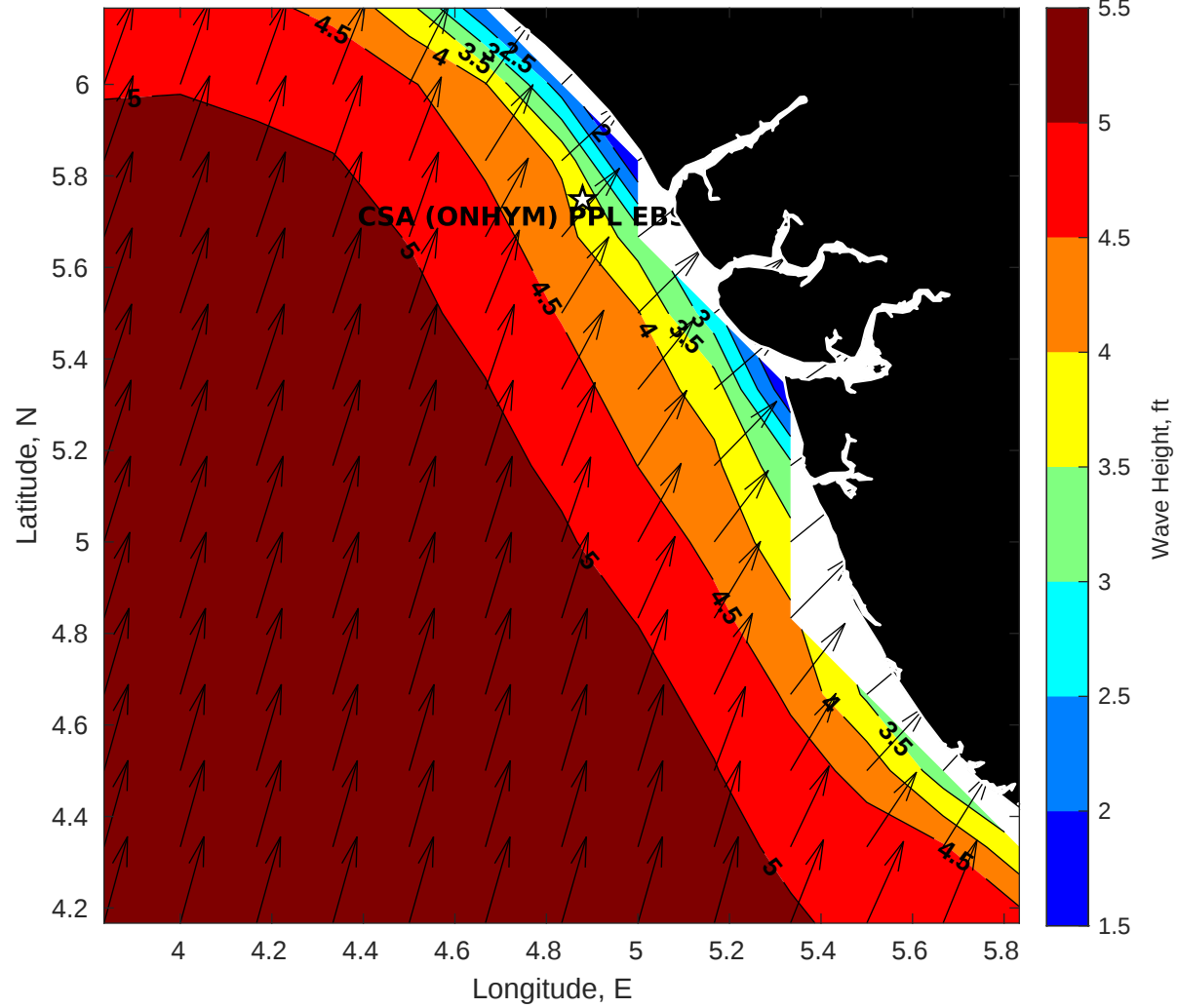
Wave Height (ft) for CSA (ONHYM) PPL EBS - Nigeria at 18-Jul-2025 09:00:00
