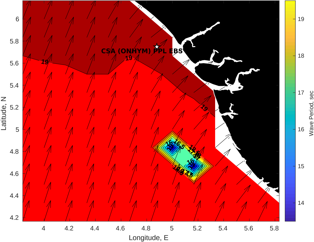
Wave Period (sec) for CSA (ONHYM) PPL EBS - Nigeria at 18-Jul-2025 09:00:00
