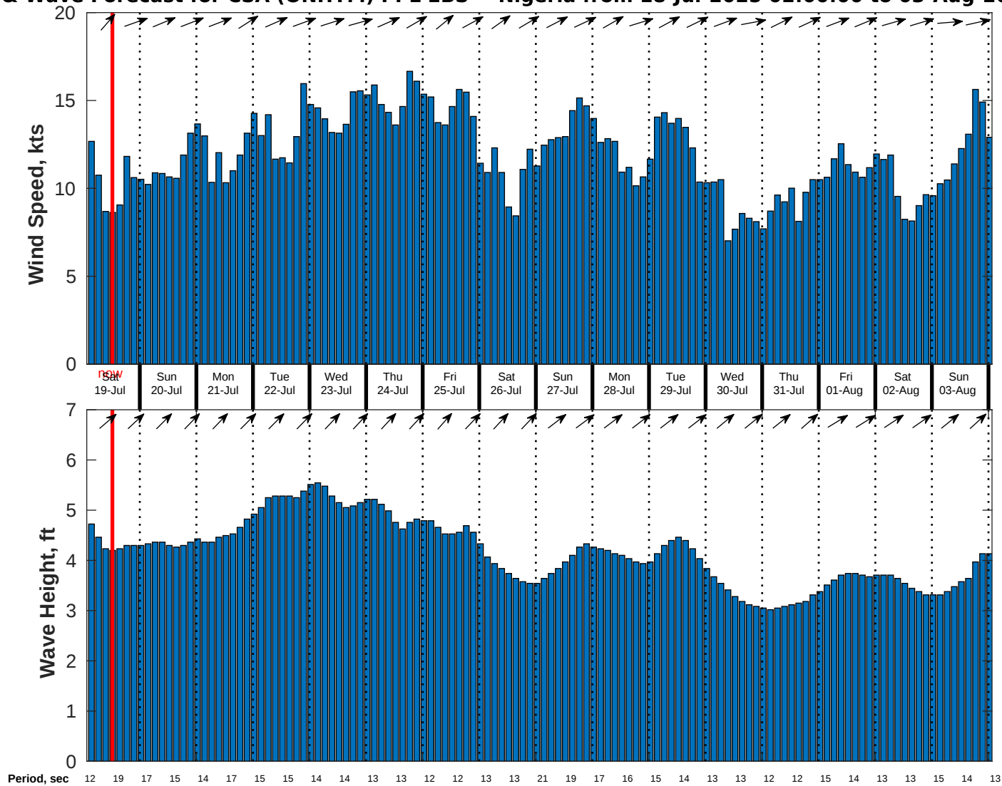
Wind & Wave Forecast for CSA (ONHYM) PPL EBS - Nigeria from 18-Jul-2025 02:00:00 to 03-Aug-2025 02:00:00
