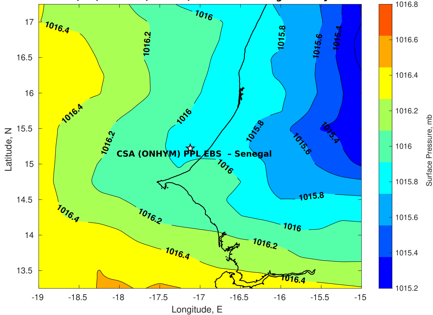
Surface Pressure (mb) for CSA (ONHYM) PPL EBS - Senegal at 20-Jul-2025 00:00:00
