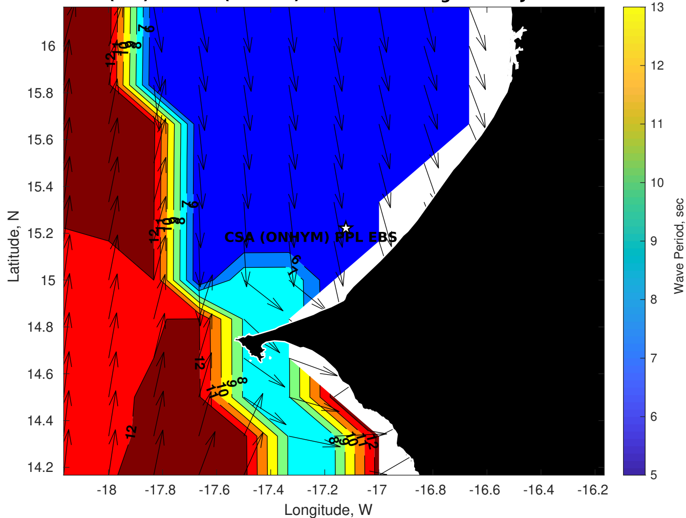
Wave Period (sec) for CSA (ONHYM) PPL EBS - Senegal at 18-Jul-2025 09:00:00
