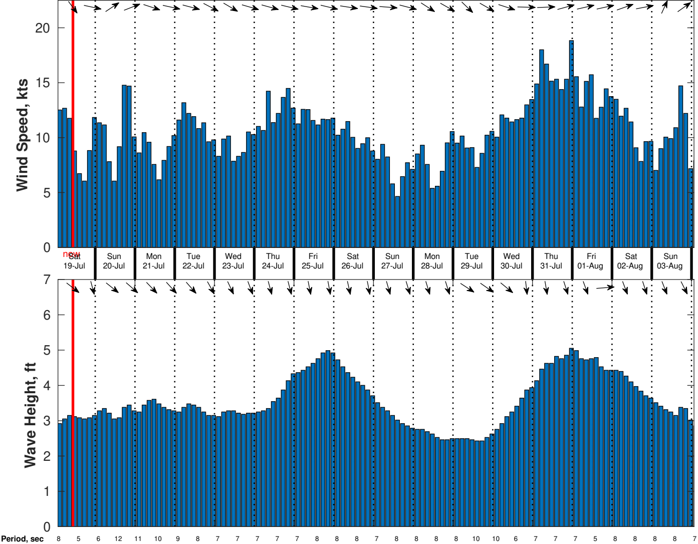
Wind & Wave Forecast for CSA (ONHYM) PPL EBS - Senegal from 18-Jul-2025 01:00:00 to 03-Aug-2025 01:00:00
