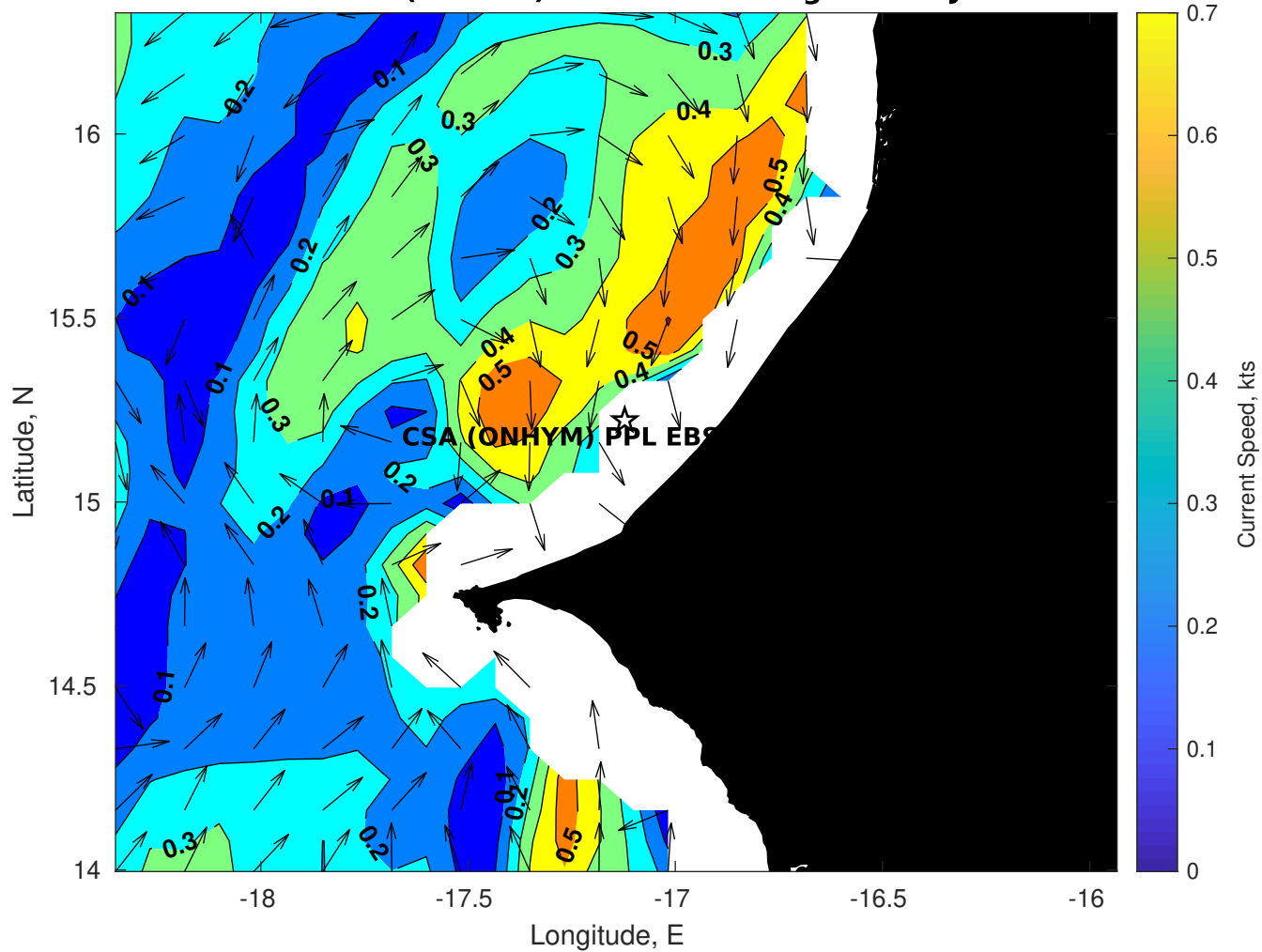
Surface Currents for CSA (ONHYM) PPL EBS - Senegal at 17-Jul-2025 00:00:00
