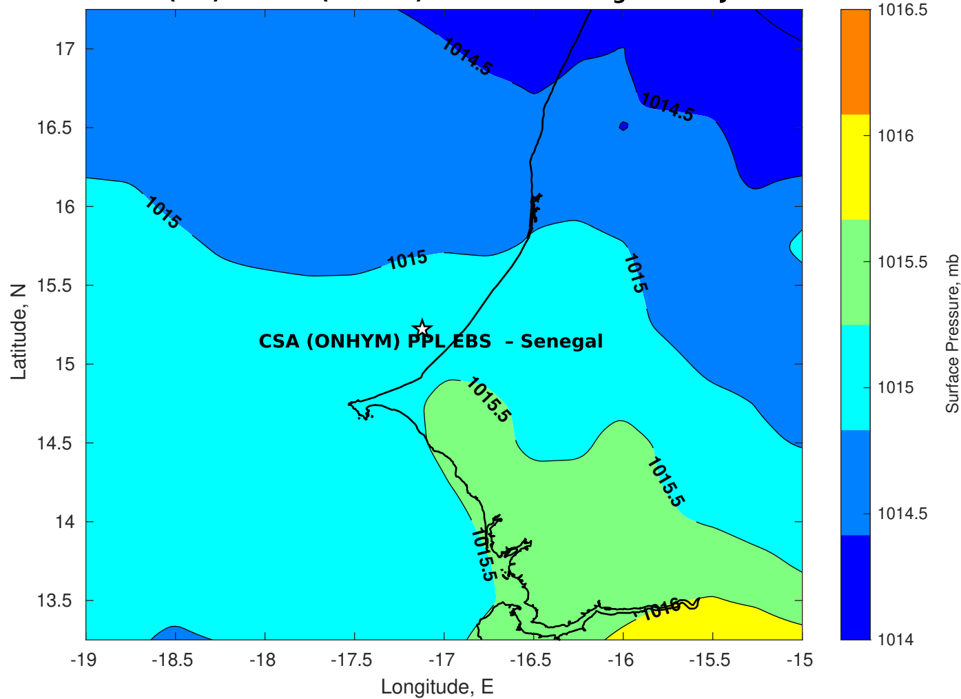
Surface Pressure (mb) for CSA (ONHYM) PPL EBS - Senegal at 19-Jul-2025 00:00:00
