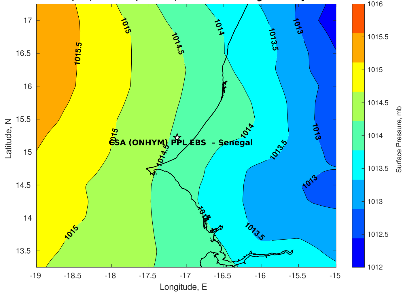
Surface Pressure (mb) for CSA (ONHYM) PPL EBS - Senegal at 18-Jul-2025 00:00:00
