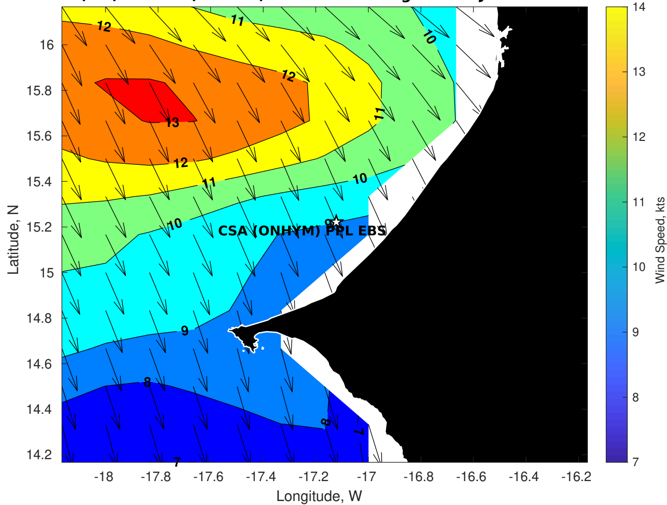
Winds (kts) for CSA (ONHYM) PPL EBS - Senegal at 18-Jul-2025 09:00:00
