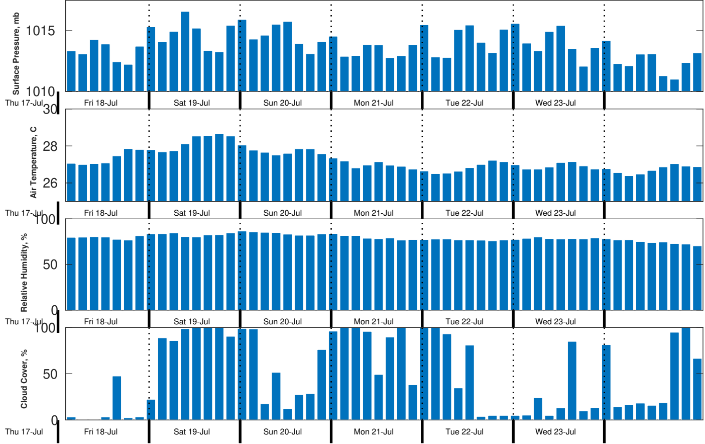
Met Forecast for CSA (ONHYM) PPL EBS - Senegal from 18-Jul-2025 00:00:00 to 25-Jul-2025 00:00:00
