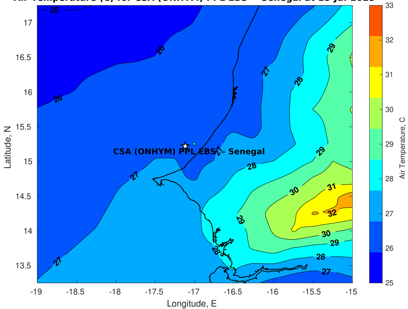
Air Temperature (C) for CSA (ONHYM) PPL EBS - Senegal at 18-Jul-2025
