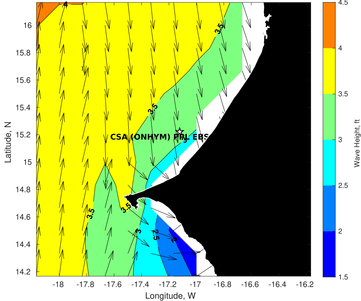
Wave Height (ft) for CSA (ONHYM) PPL EBS - Senegal at 18-Jul-2025 09:00:00
