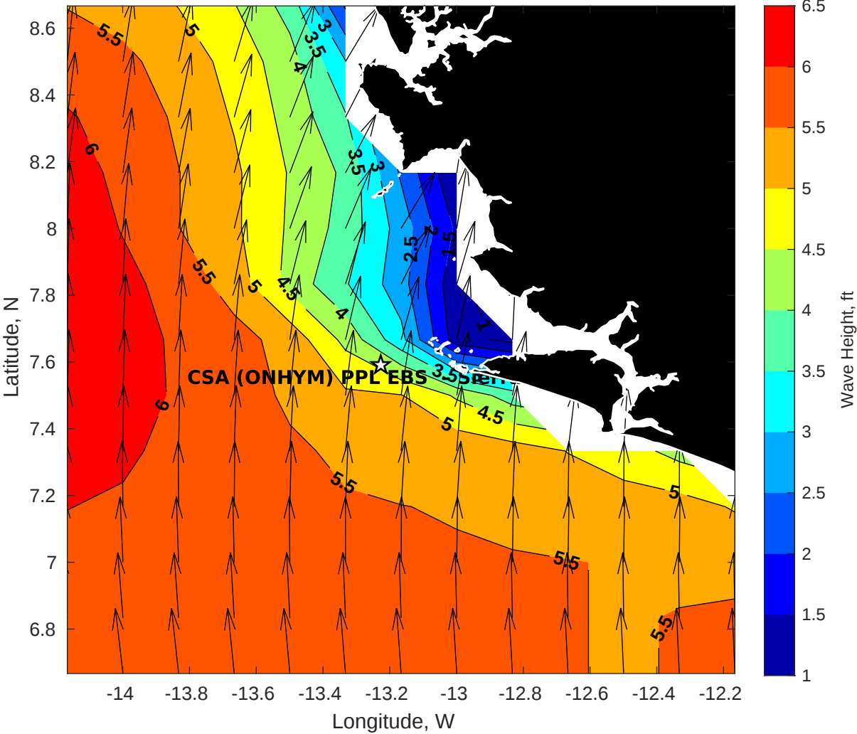
Wave Height (ft) for CSA (ONHYM) PPL EBS - Sierra Leone at 18-Jul-2025 09:00:00
