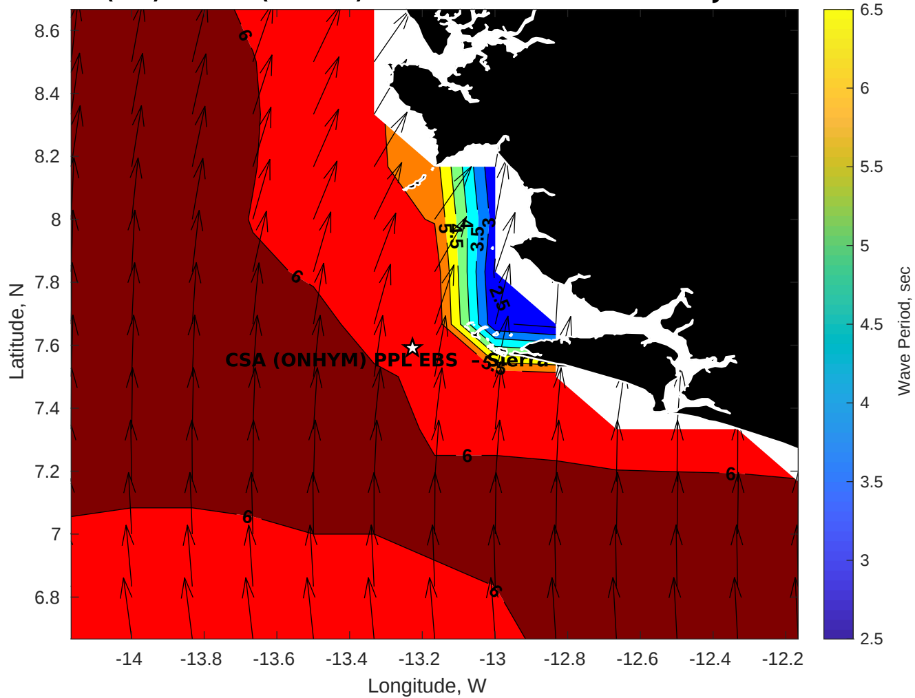
Wave Period (sec) for CSA (ONHYM) PPL EBS - Sierra Leone at 18-Jul-2025 09:00:00
