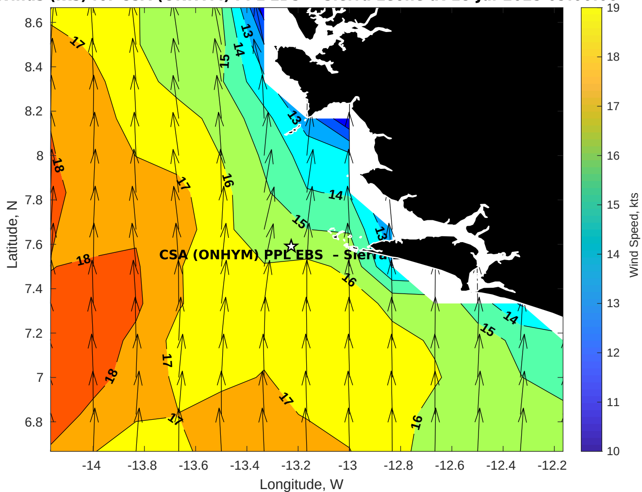
Winds (kts) for CSA (ONHYM) PPL EBS - Sierra Leone at 18-Jul-2025 09:00:00
