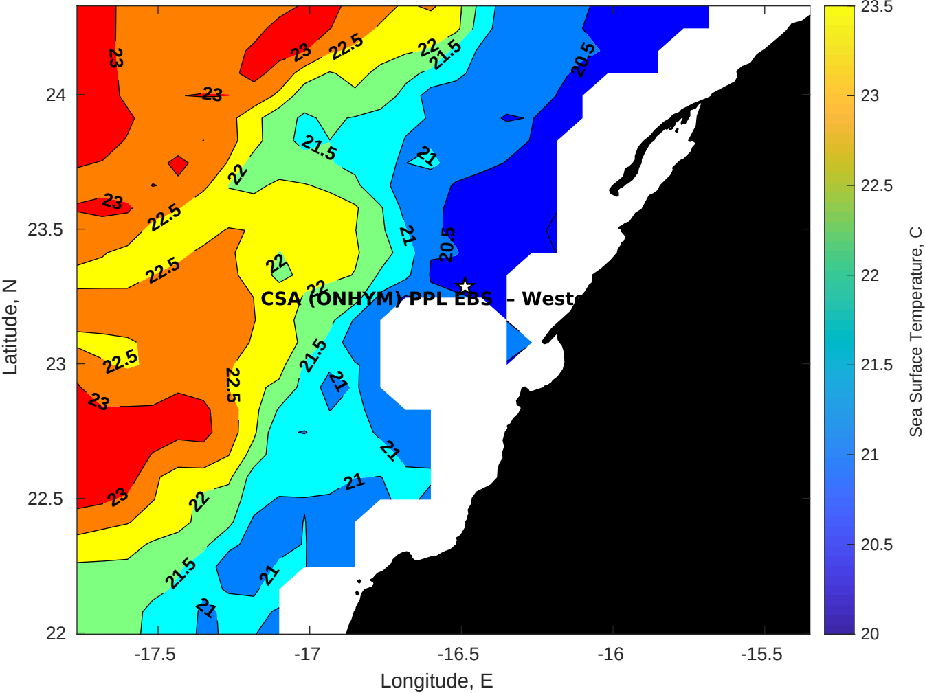
SST for CSA (ONHYM) PPL EBS - Western Sahara at 17-Jul-2025 00:00:00
