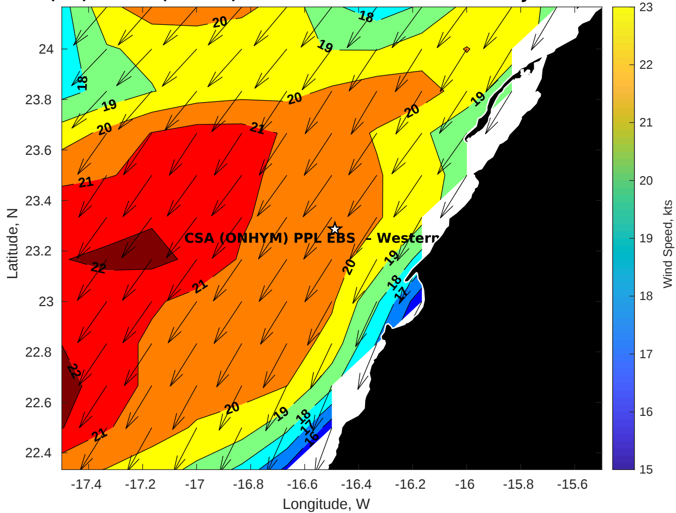
Winds (kts) for CSA (ONHYM) PPL EBS - Western Sahara at 18-Jul-2025 09:00:00
