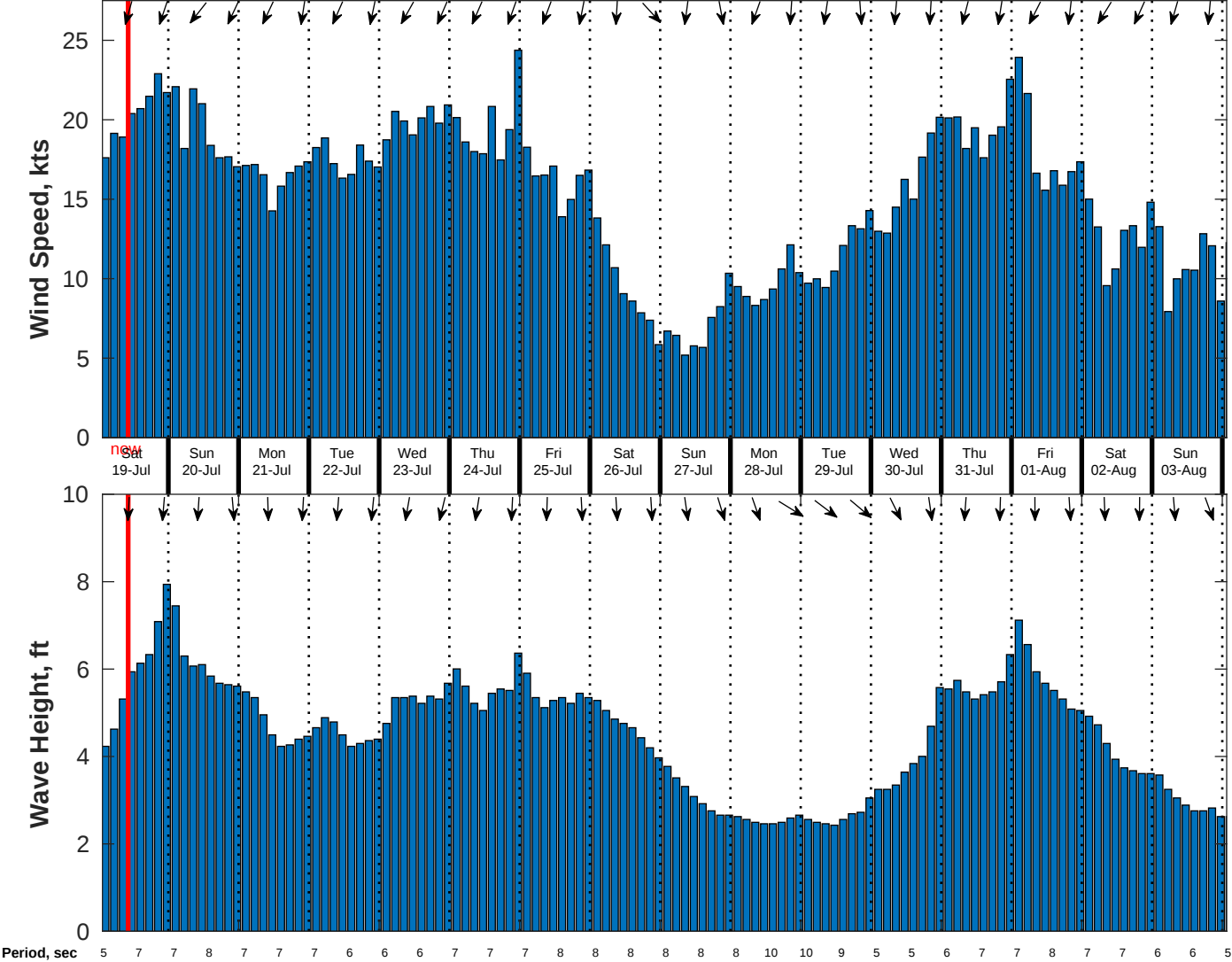
Wind & Wave Forecast for CSA (ONHYM) PPL EBS - Western Sahara from 18-Jul-2025 01:00:00 to 03-Aug-2025 01:00:00
