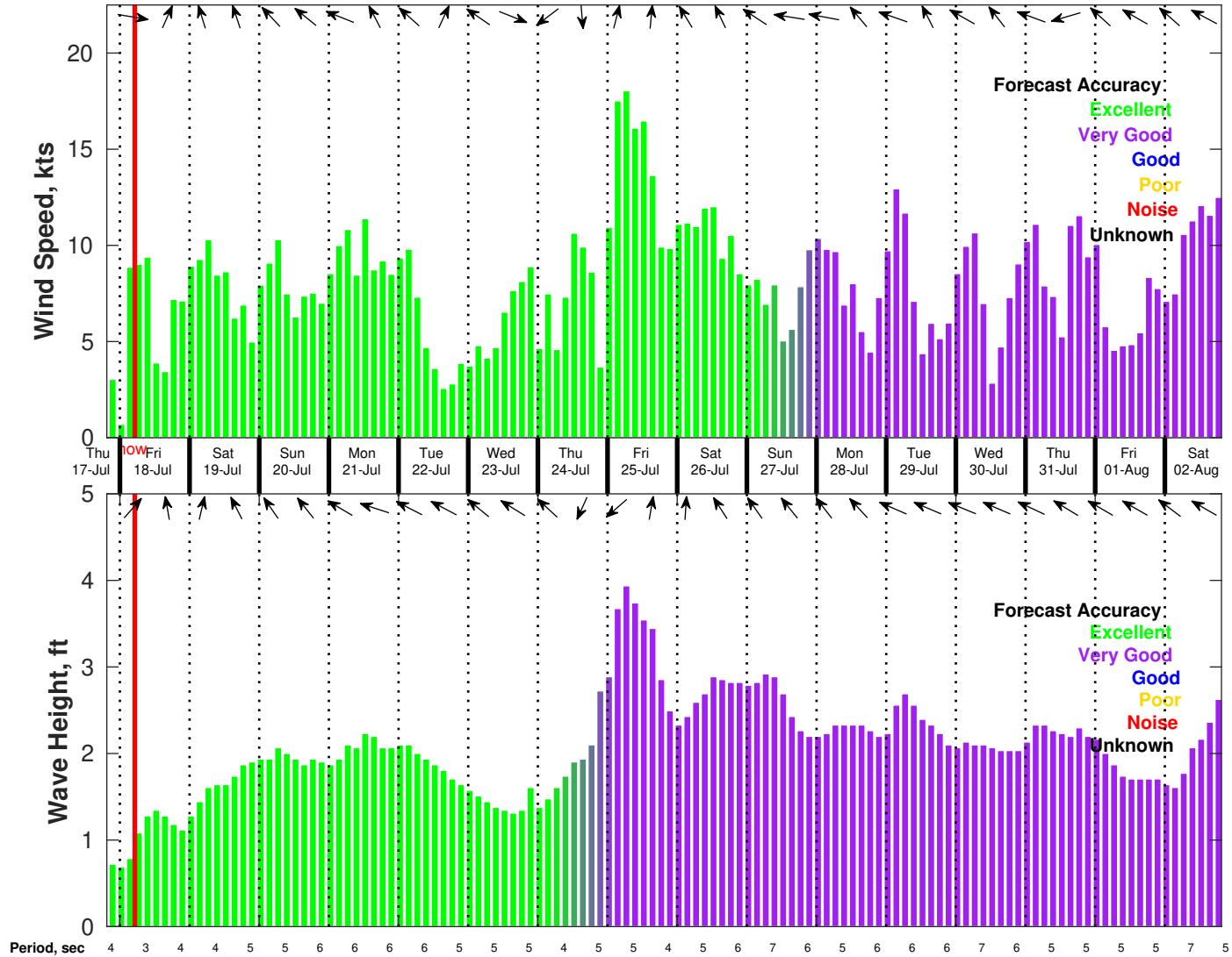
Wind & Wave Forecast for CTI Enbridge Kaskida & Tiber PPL Geotechnical from 17-Jul-2025 20:00:00 to 02-Aug-2025 20:00:00
