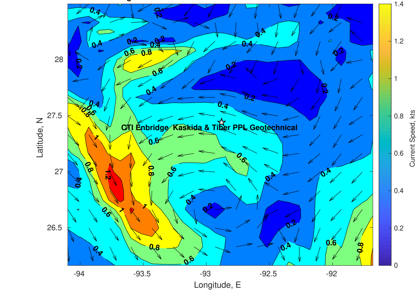
Surface Currents for CTI Enbridge Kaskida & Tiber PPL Geotechnical at 17-Jul-2025 00:00:00
