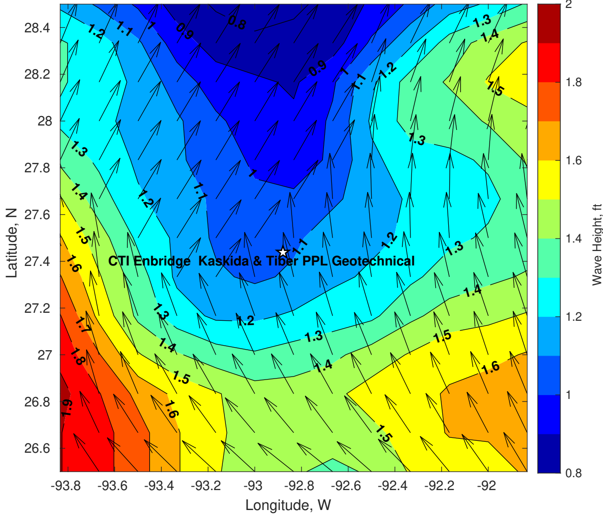
Wave Height (ft) for CTI Enbridge Kaskida & Tiber PPL Geotechnical at 18-Jul-2025 09:00:00
