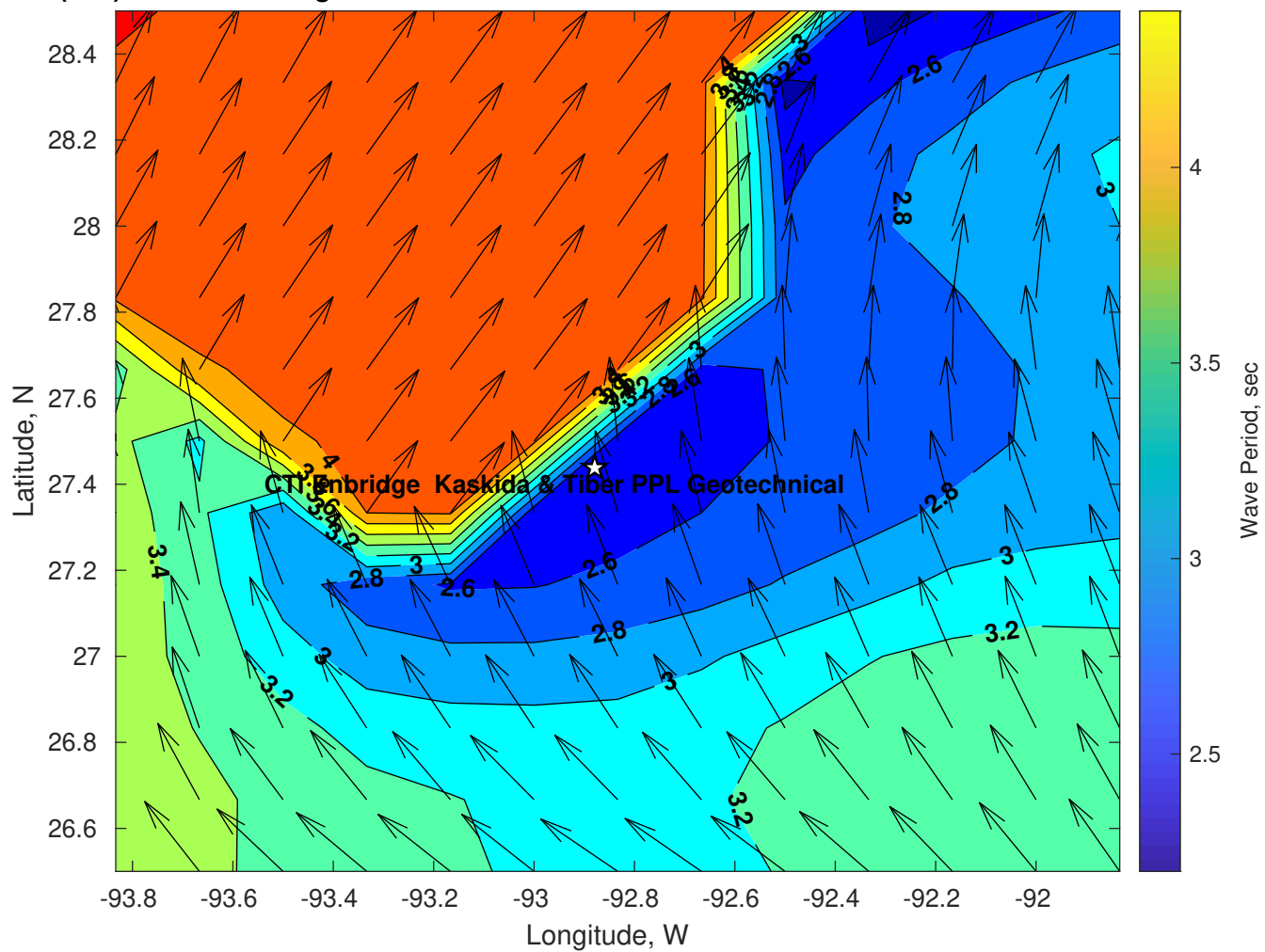
Wave Period (sec) for CTI Enbridge Kaskida & Tiber PPL Geotechnical at 18-Jul-2025 09:00:00
