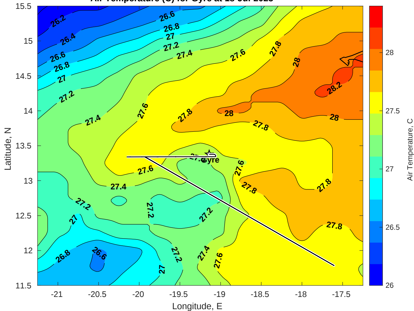
Air Temperature (C) for Gyre at 18-Jul-2025
