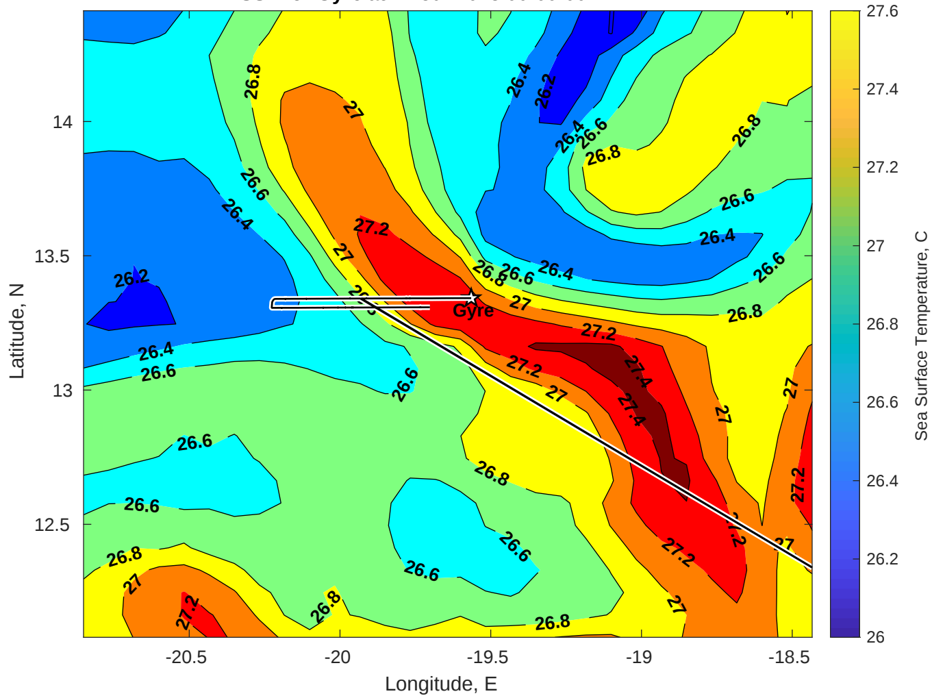
SST for Gyre at 17-Jul-2025 00:00:00
