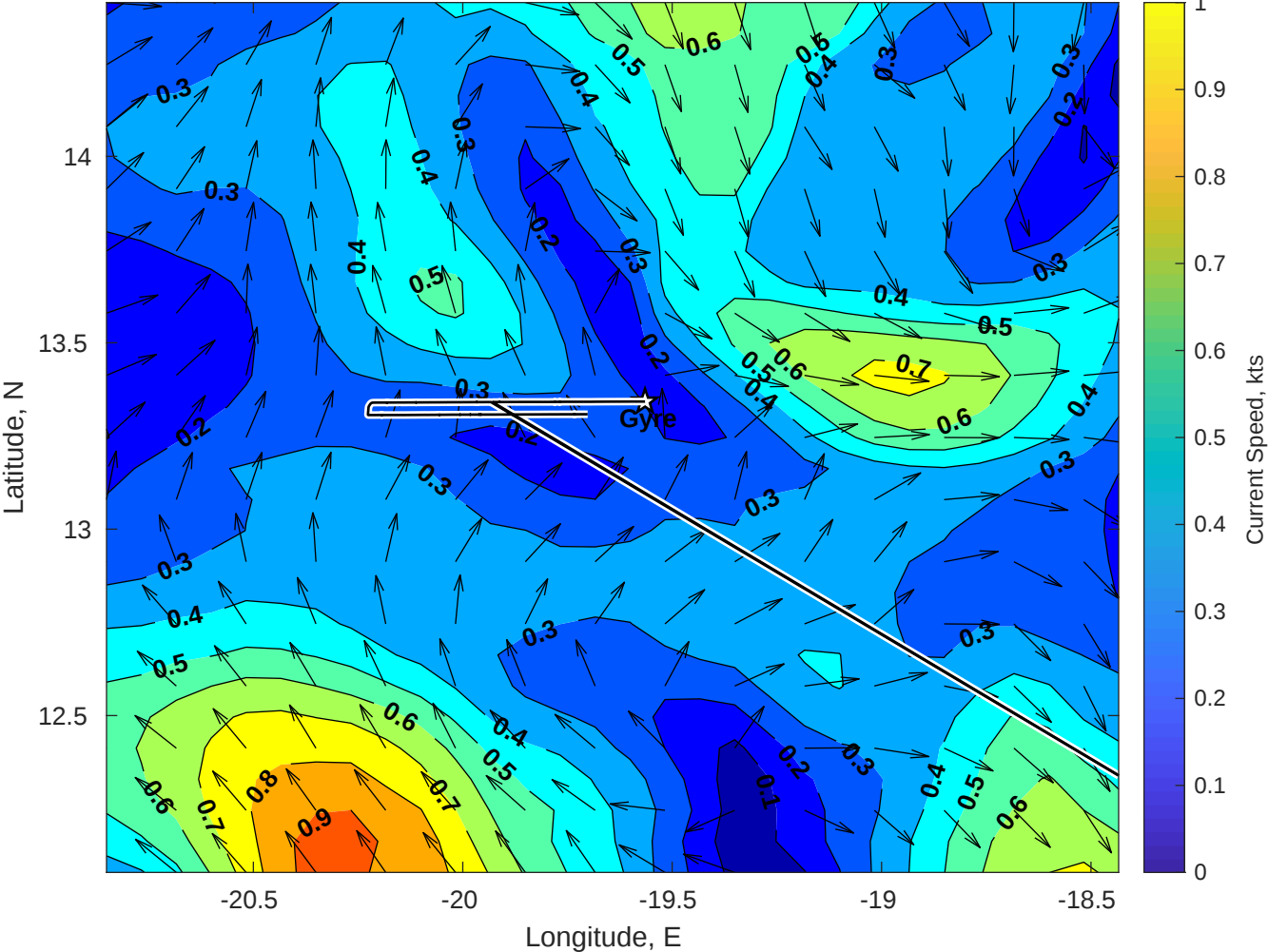
Surface Currents for Gyre at 17-Jul-2025 00:00:00
