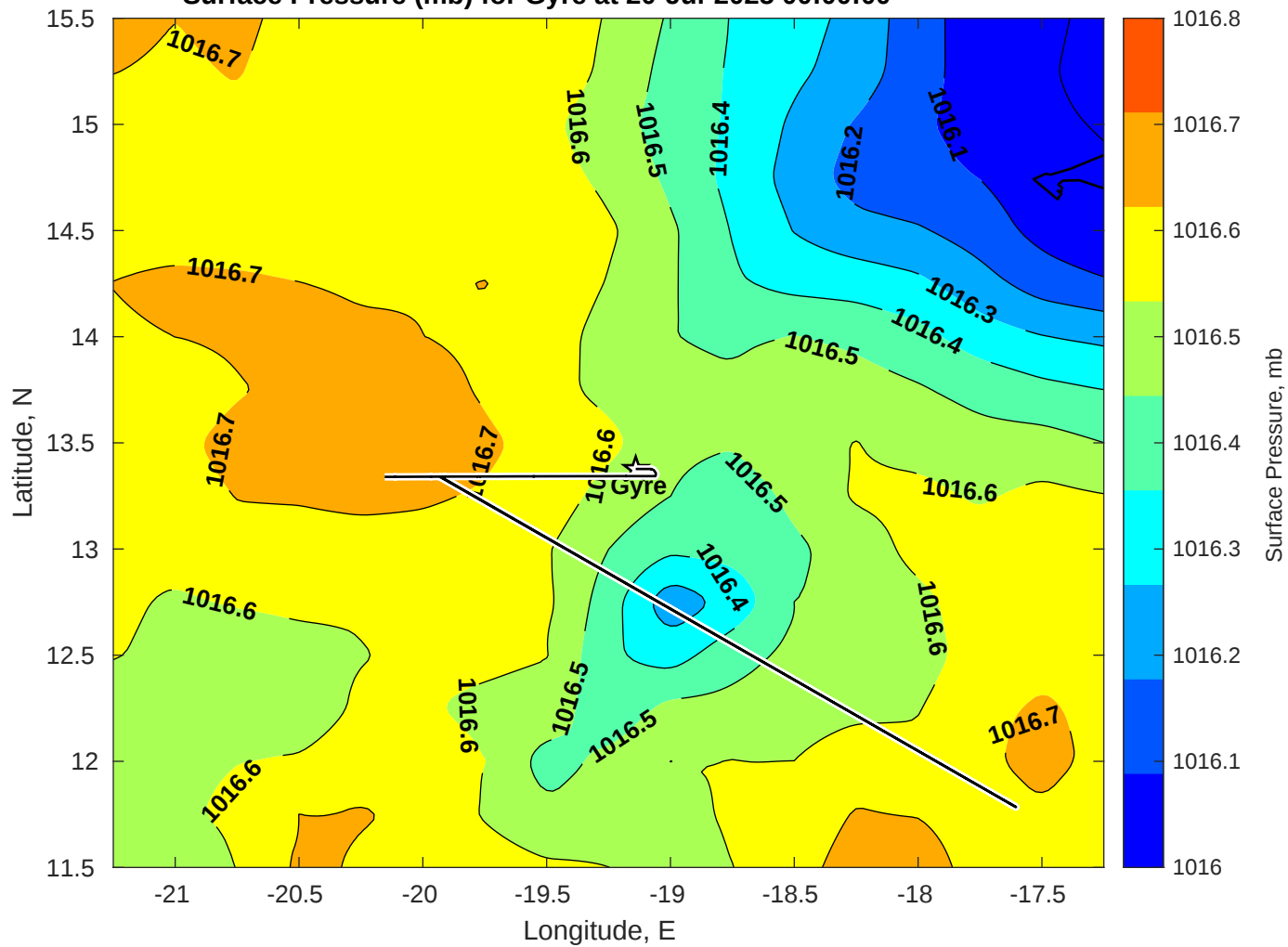
Surface Pressure (mb) for Gyre at 20-Jul-2025 00:00:00
