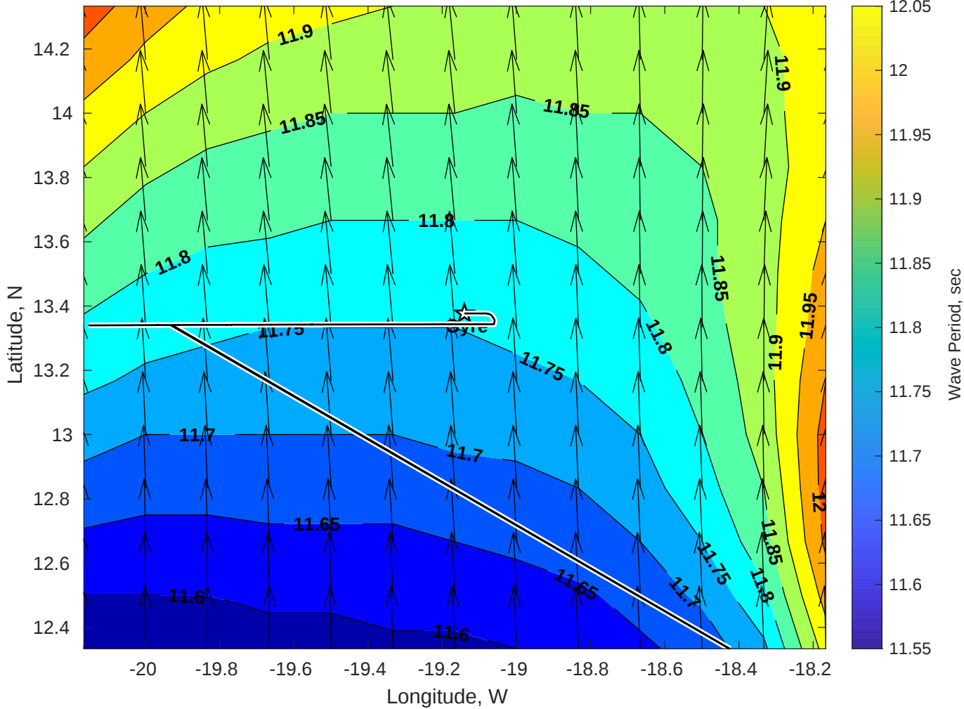
Wave Period (sec) for Gyre at 18-Jul-2025 09:00:00
