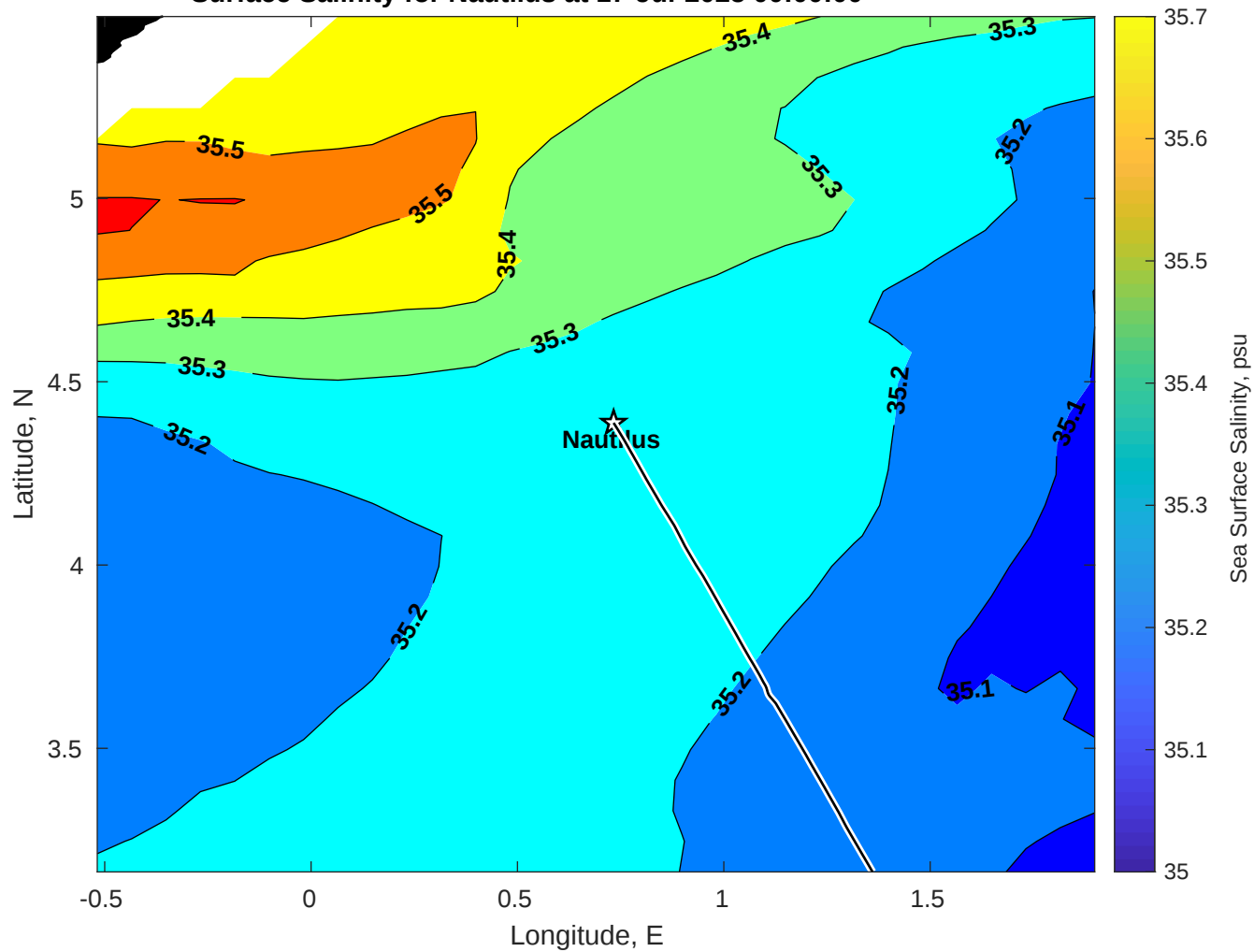
Surface Salinity for Nautilus at 17-Jul-2025 00:00:00
