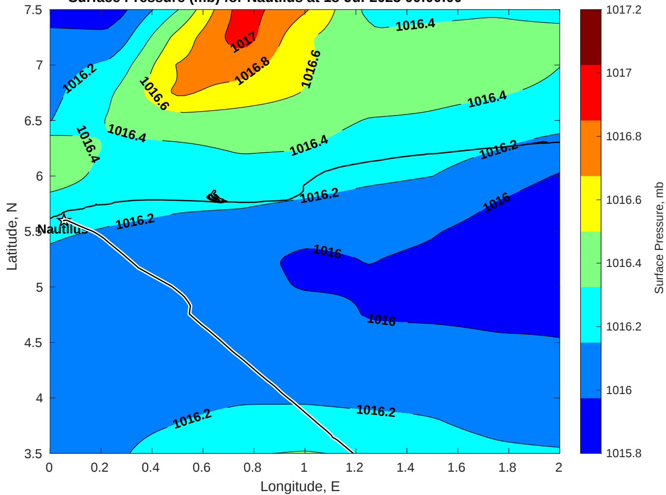
Surface Pressure (mb) for Nautilus at 18-Jul-2025 00:00:00
