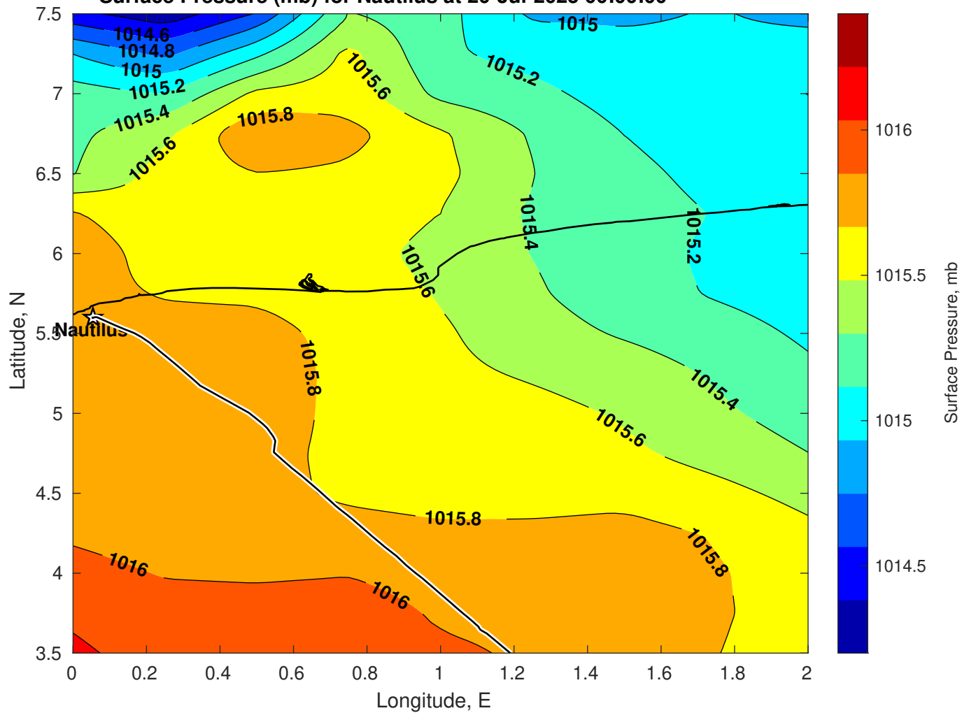
Surface Pressure (mb) for Nautilus at 20-Jul-2025 00:00:00
