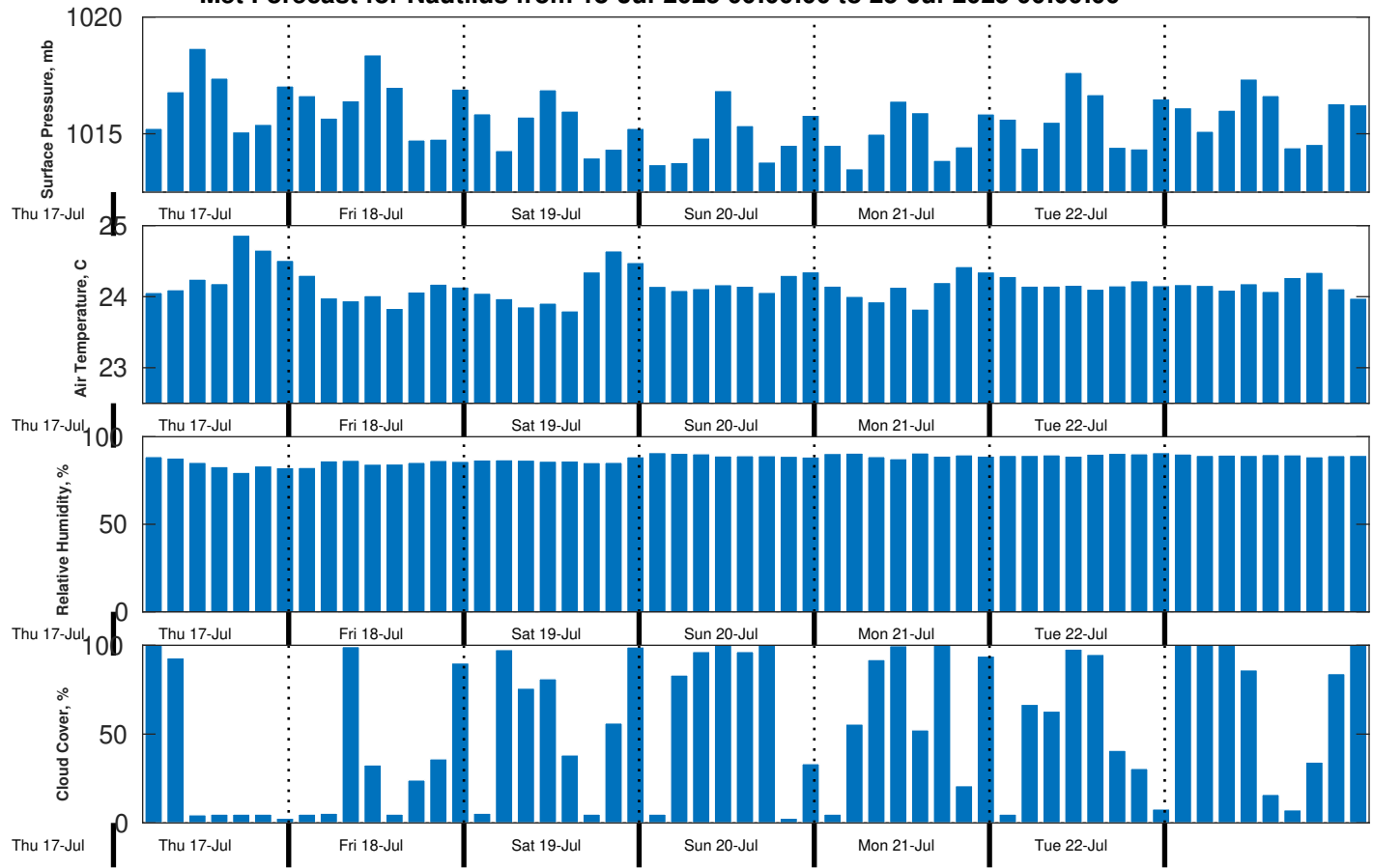
Met Forecast for Nautilus from 18-Jul-2025 00:00:00 to 25-Jul-2025 00:00:00
