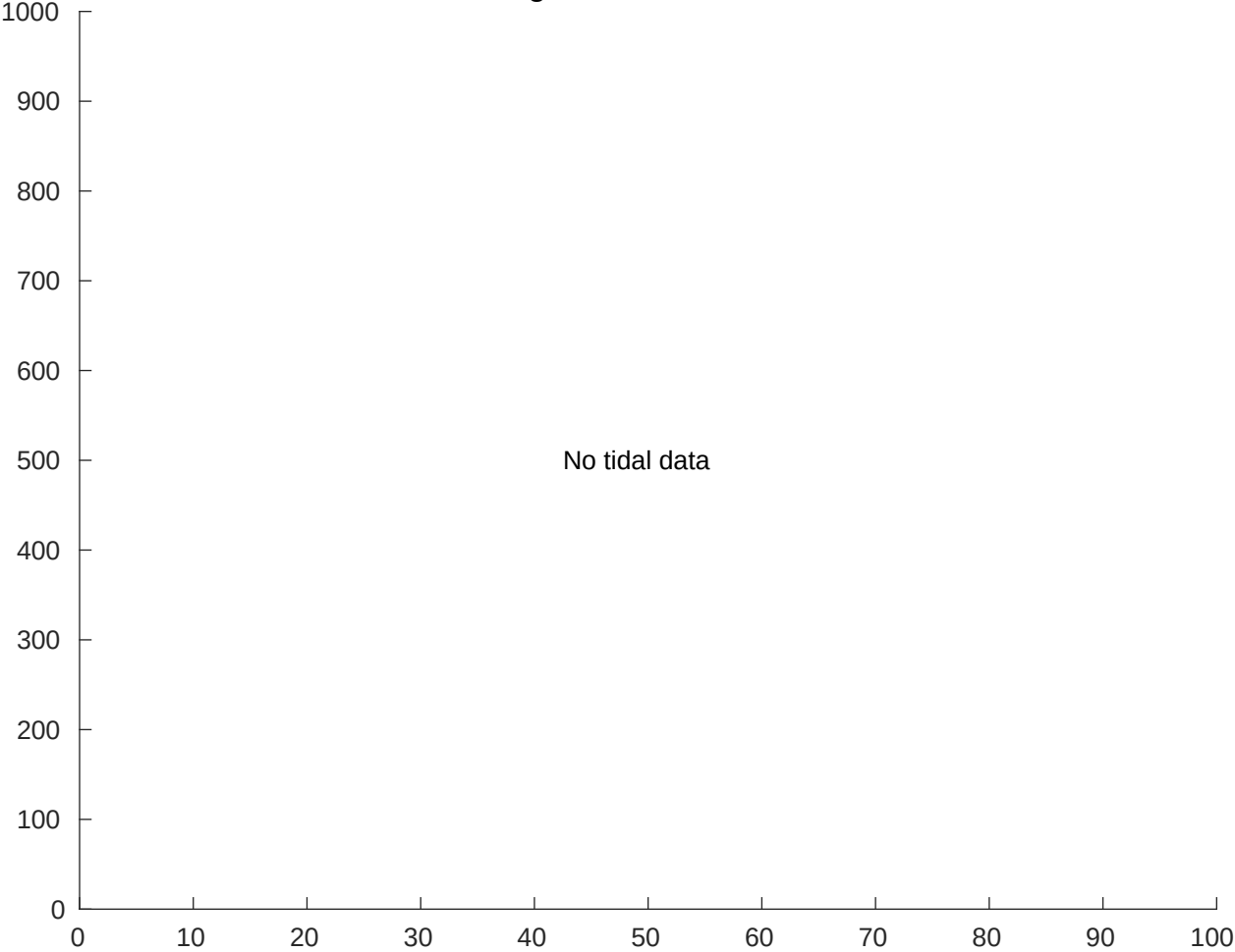
Tidal Currents and Heights for Nautilus at 20250718
