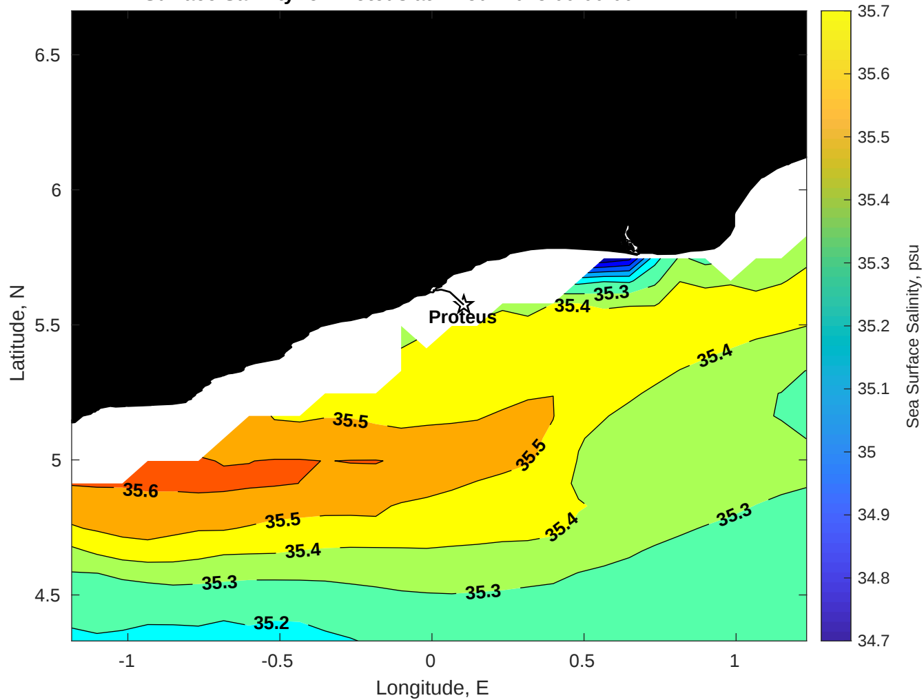
Surface Salinity for Proteus at 17-Jul-2025 00:00:00
