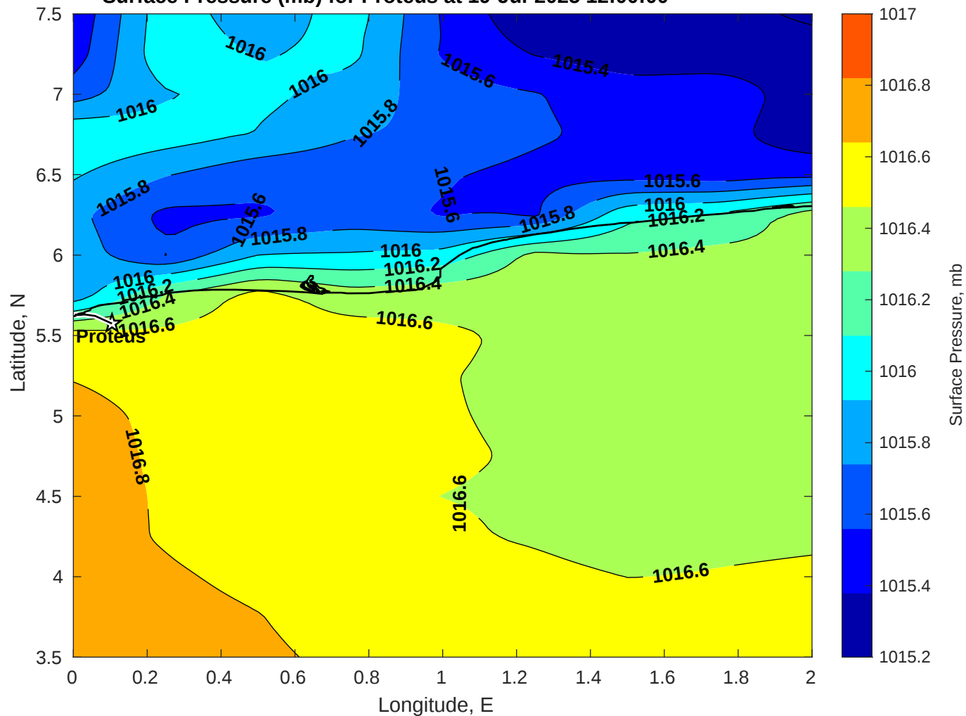
Surface Pressure (mb) for Proteus at 19-Jul-2025 12:00:00
