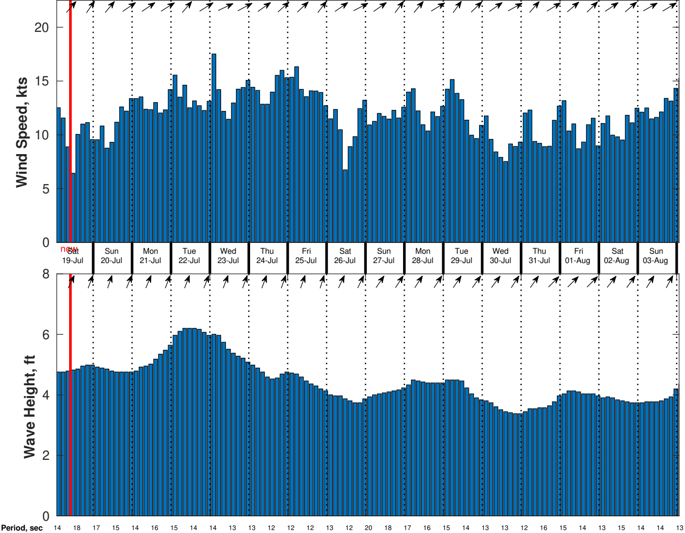
Wind & Wave Forecast for Proteus from 18-Jul-2025 01:00:00 to 03-Aug-2025 01:00:00
