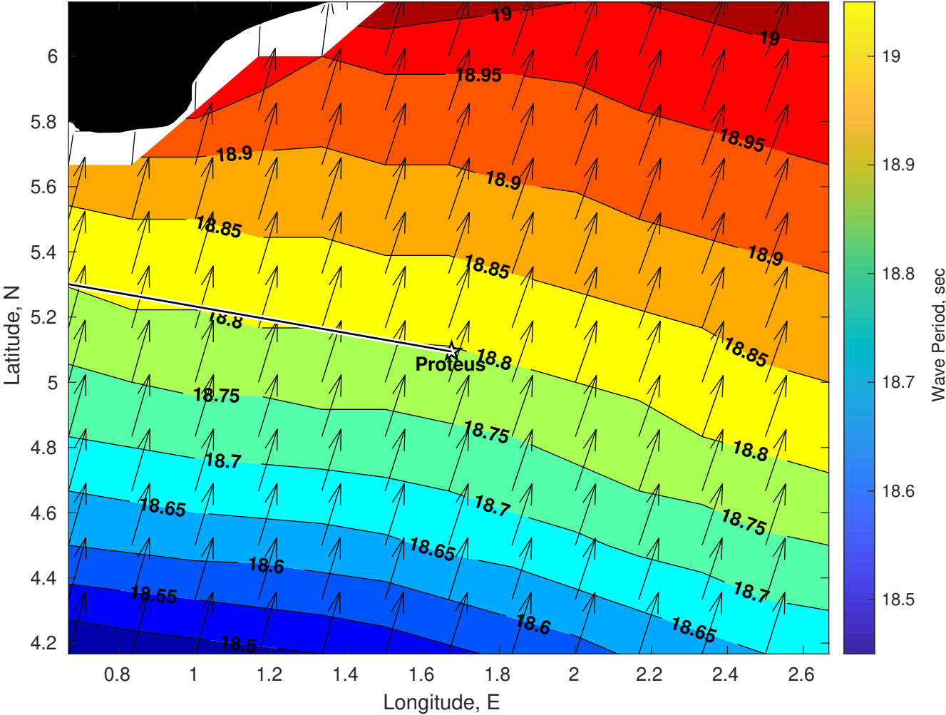
Wave Period (sec) for Proteus at 18-Jul-2025 09:00:00
