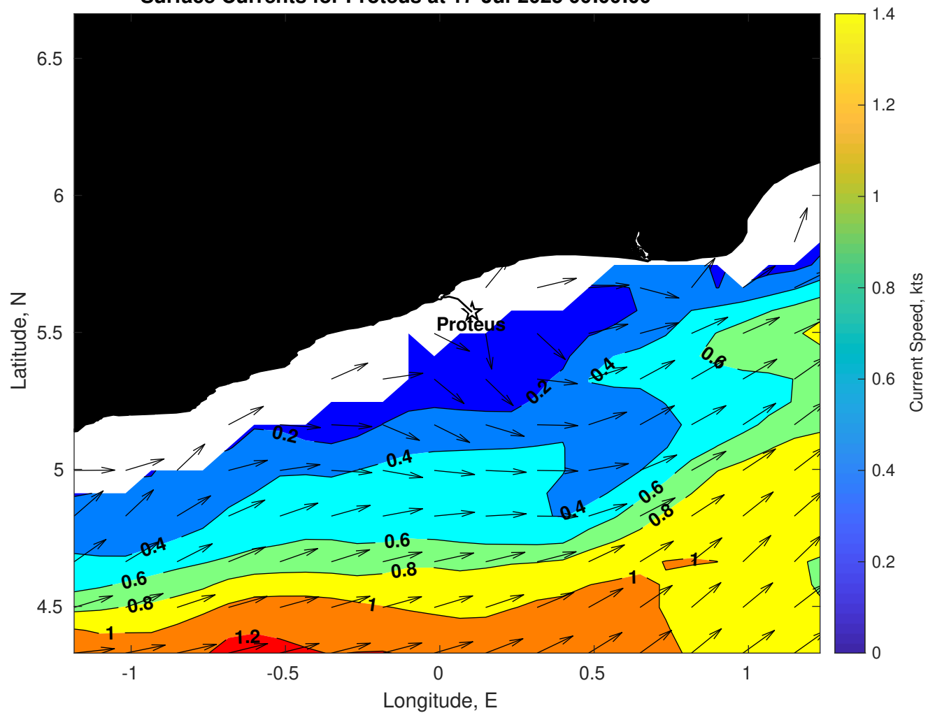
Surface Currents for Proteus at 17-Jul-2025 00:00:00
