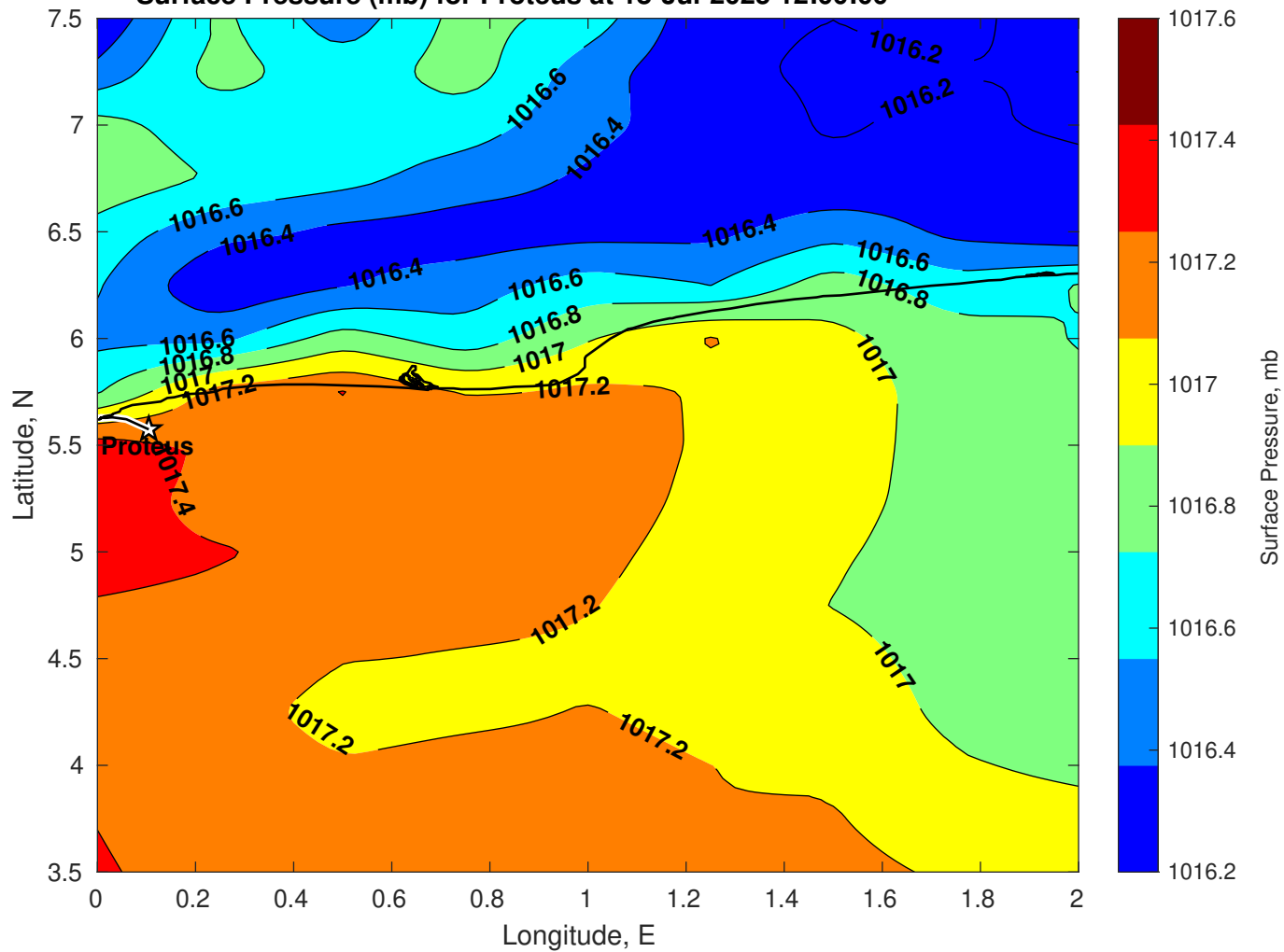
Surface Pressure (mb) for Proteus at 18-Jul-2025 12:00:00
