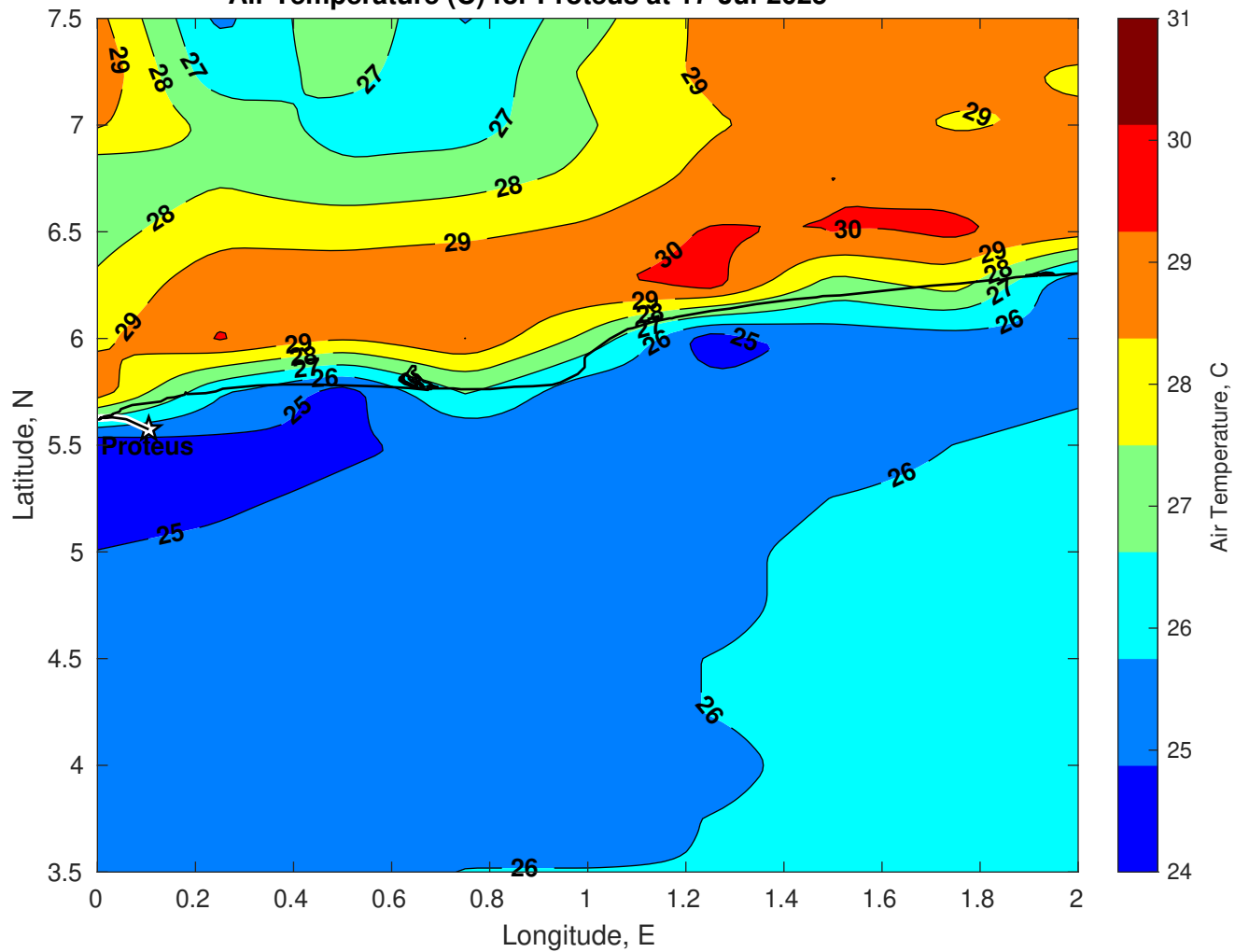
Air Temperature (C) for Proteus at 17-Jul-2025
