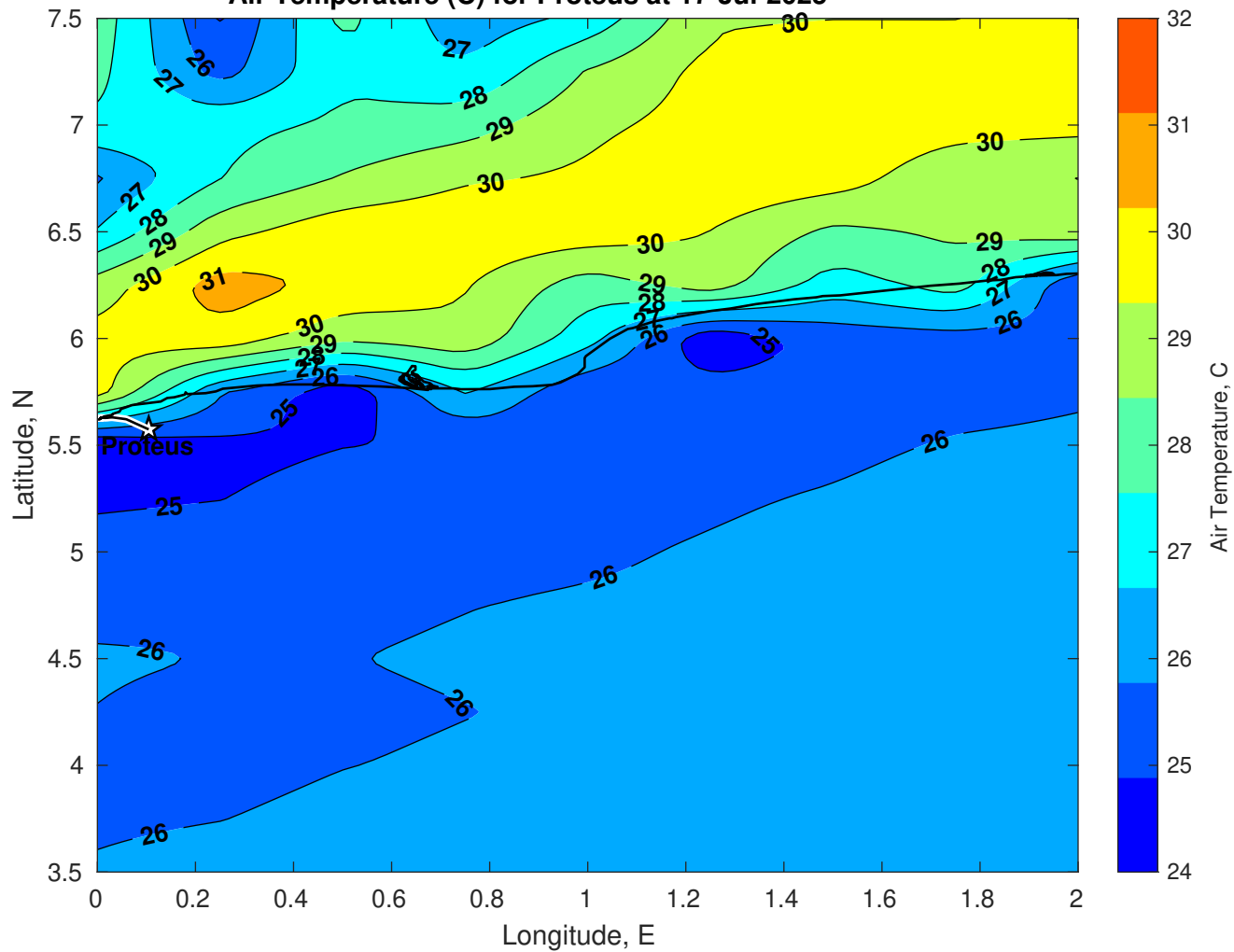
Air Temperature (C) for Proteus at 17-Jul-2025
