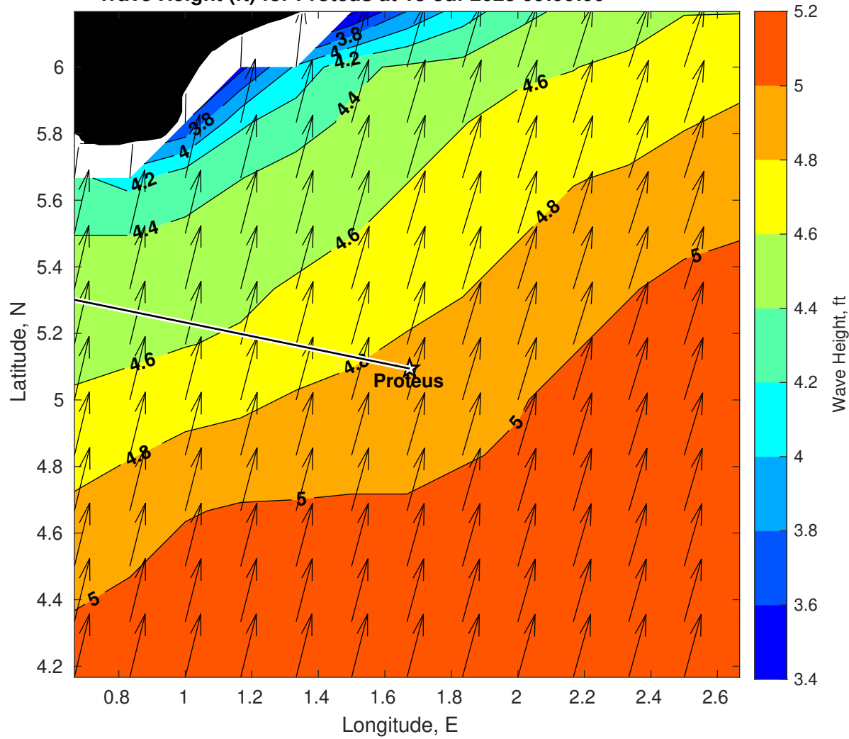
Wave Height (ft) for Proteus at 18-Jul-2025 09:00:00
