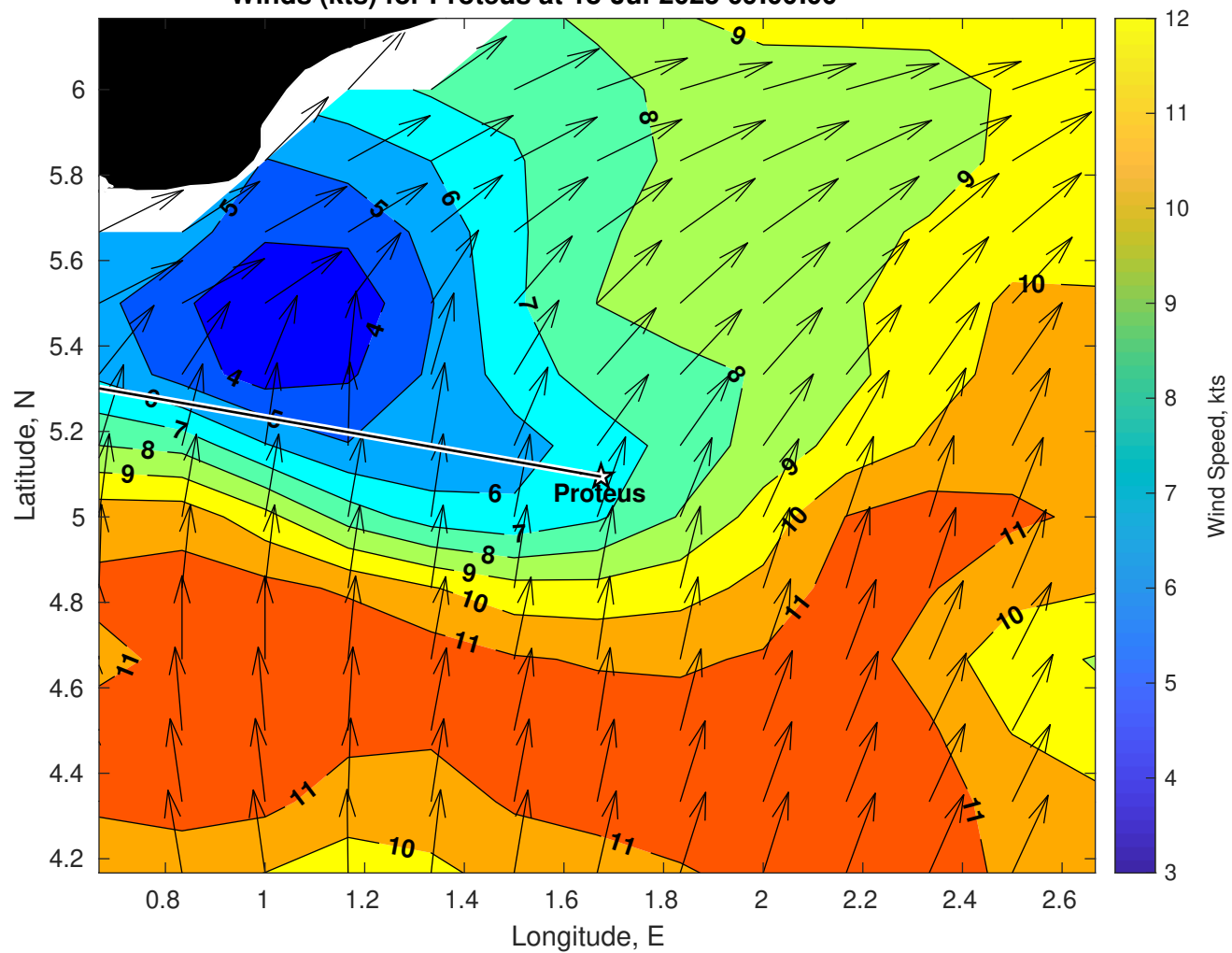
Winds (kts) for Proteus at 18-Jul-2025 09:00:00
