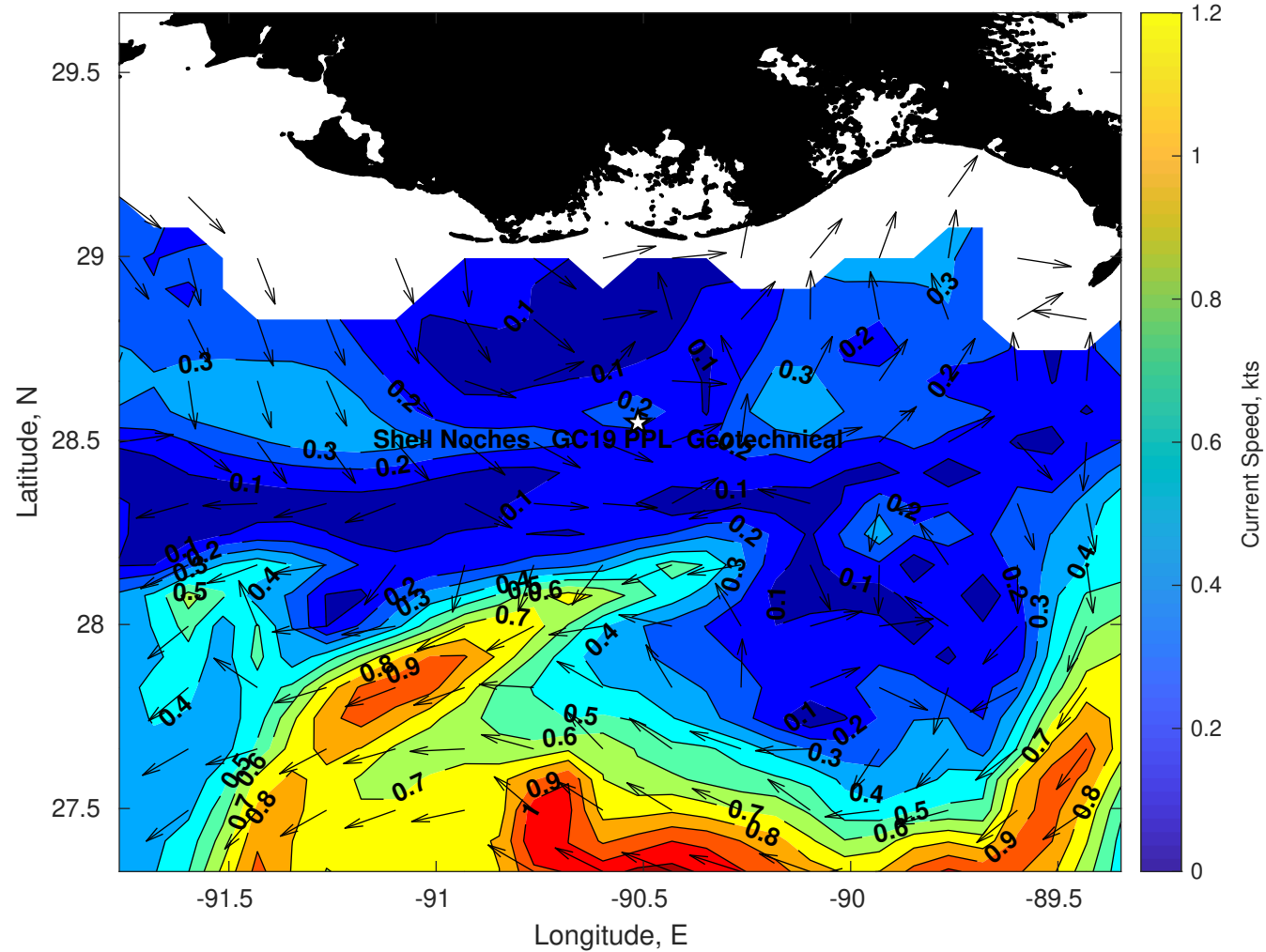
Surface Currents for Shell Noches GC19 PPL Geotechnical at 17-Jul-2025 00:00:00
