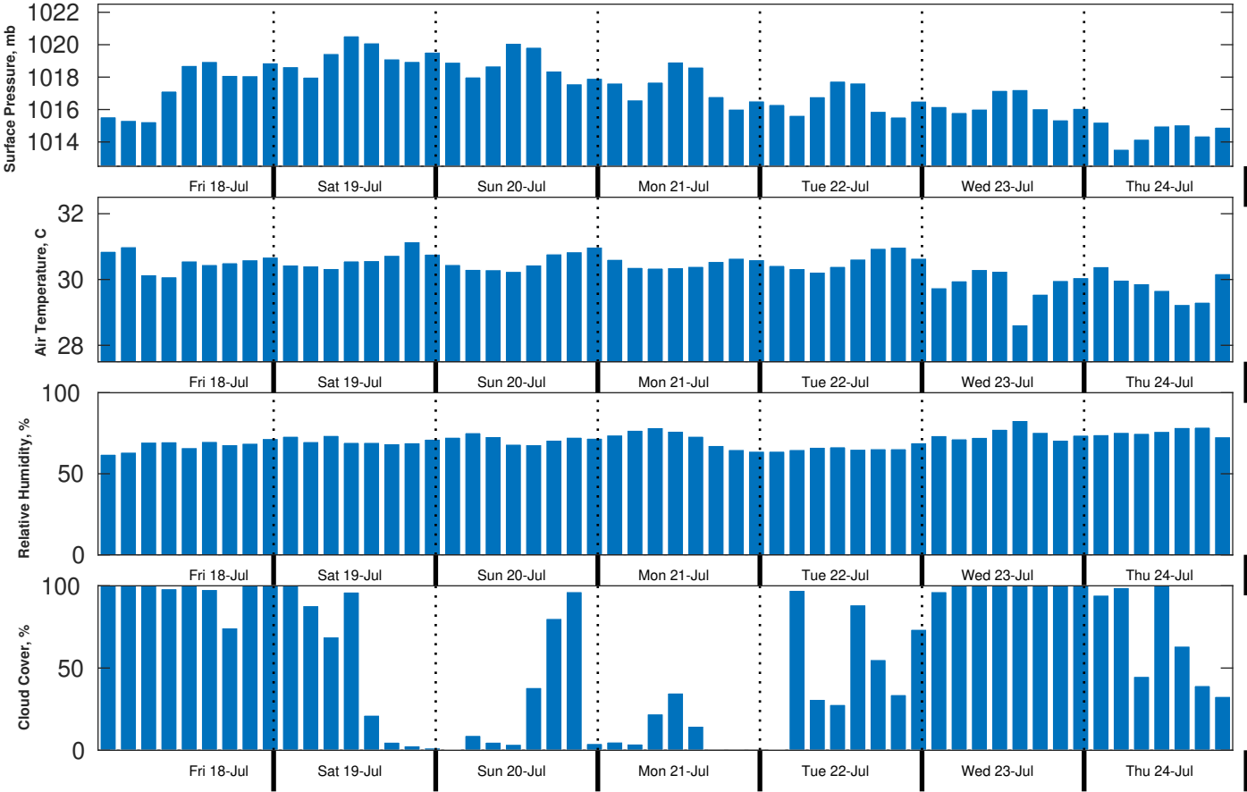
Met Forecast for Shell Noches GC19 PPL Geotechnical from 18-Jul-2025 00:00:00 to 25-Jul-2025 00:00:00
