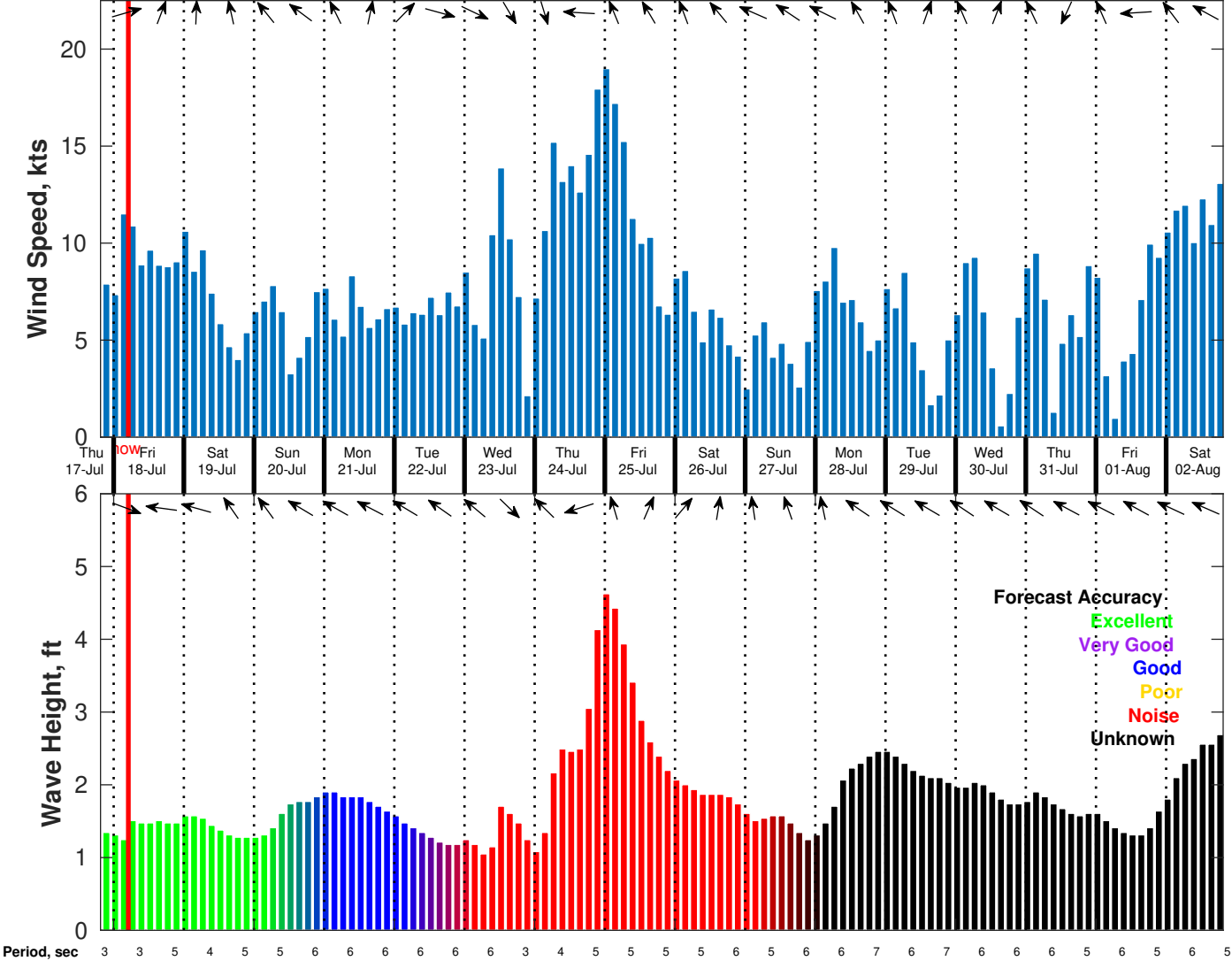
Wind & Wave Forecast for Shell Noches GC19 PPL Geotechnical from 17-Jul-2025 20:00:00 to 02-Aug-2025 20:00:00
