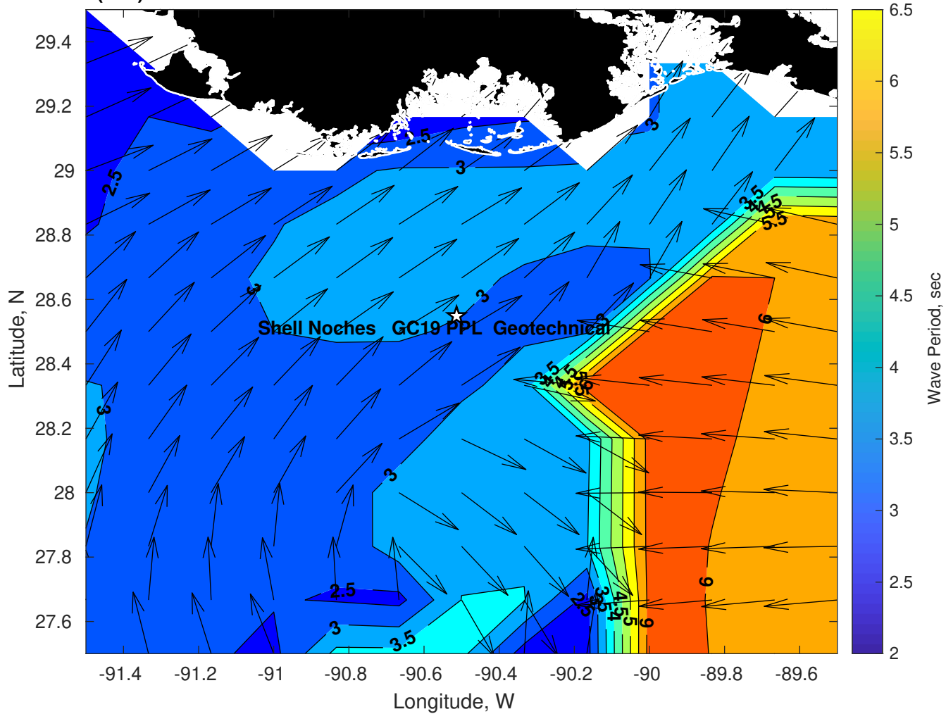
Wave Period (sec) for Shell Noches GC19 PPL Geotechnical at 18-Jul-2025 09:00:00
