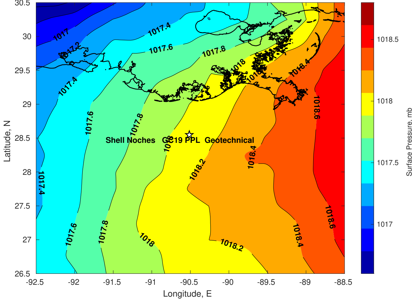
Surface Pressure (mb) for Shell Noches GC19 PPL Geotechnical at 19-Jul-2025 00:00:00
