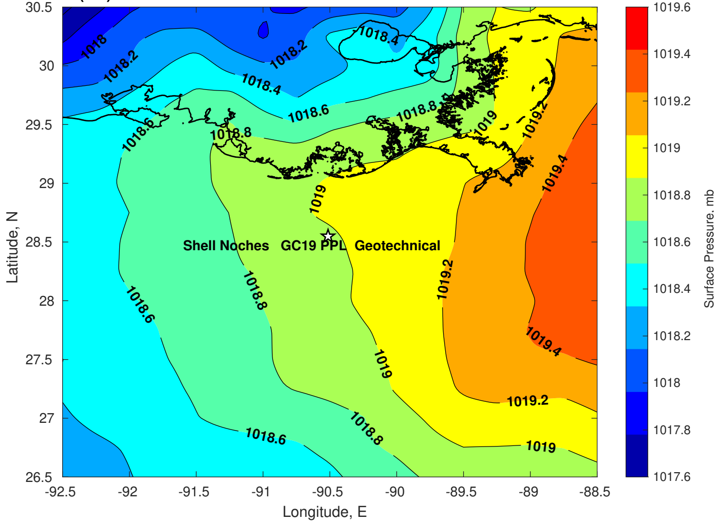
Surface Pressure (mb) for Shell Noches GC19 PPL Geotechnical at 20-Jul-2025 00:00:00
