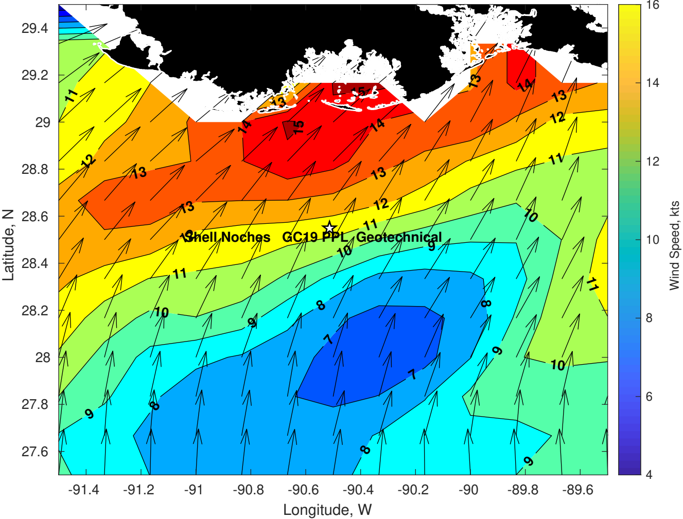
Winds (kts) for Shell Noches GC19 PPL Geotechnical at 18-Jul-2025 09:00:00
