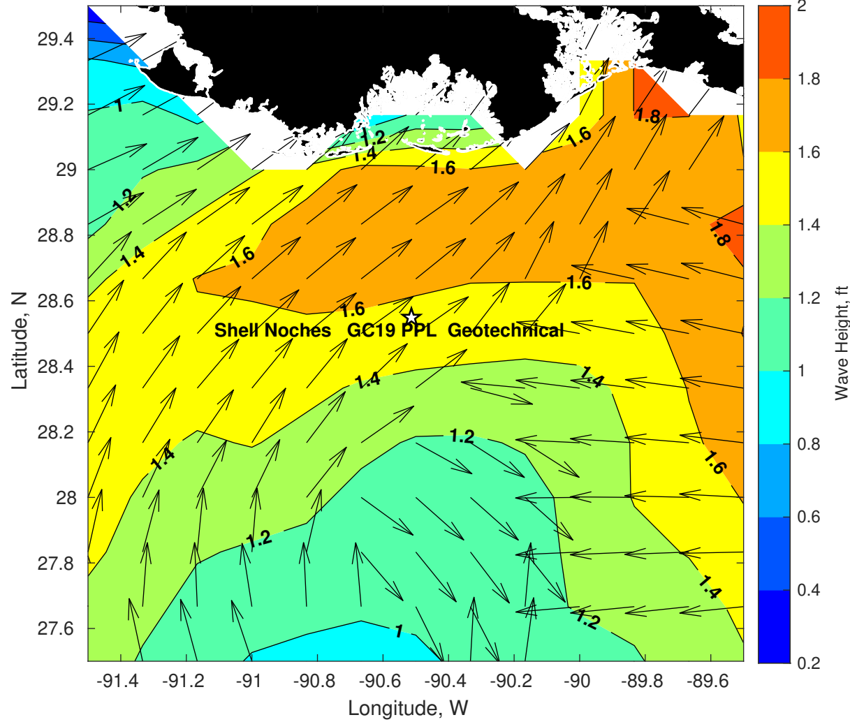
Wave Height (ft) for Shell Noches GC19 PPL Geotechnical at 18-Jul-2025 09:00:00
