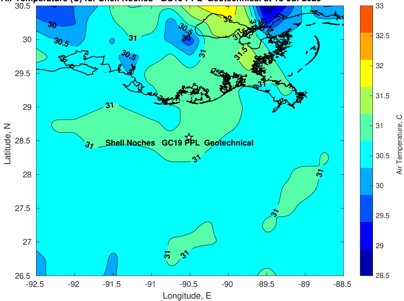
Air Temperature (C) for Shell Noches GC19 PPL Geotechnical at 18-Jul-2025
