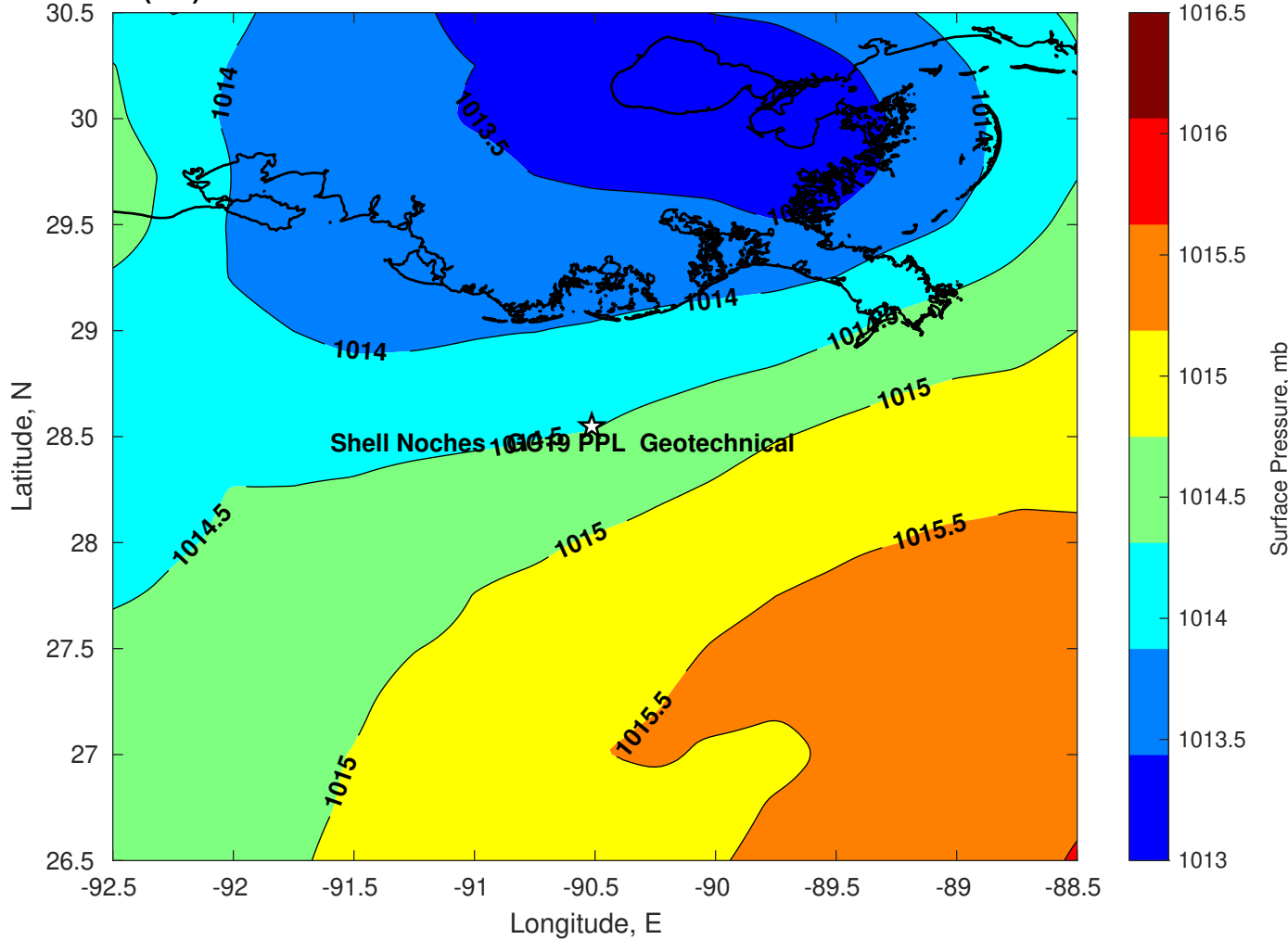
Surface Pressure (mb) for Shell Noches GC19 PPL Geotechnical at 18-Jul-2025 00:00:00
