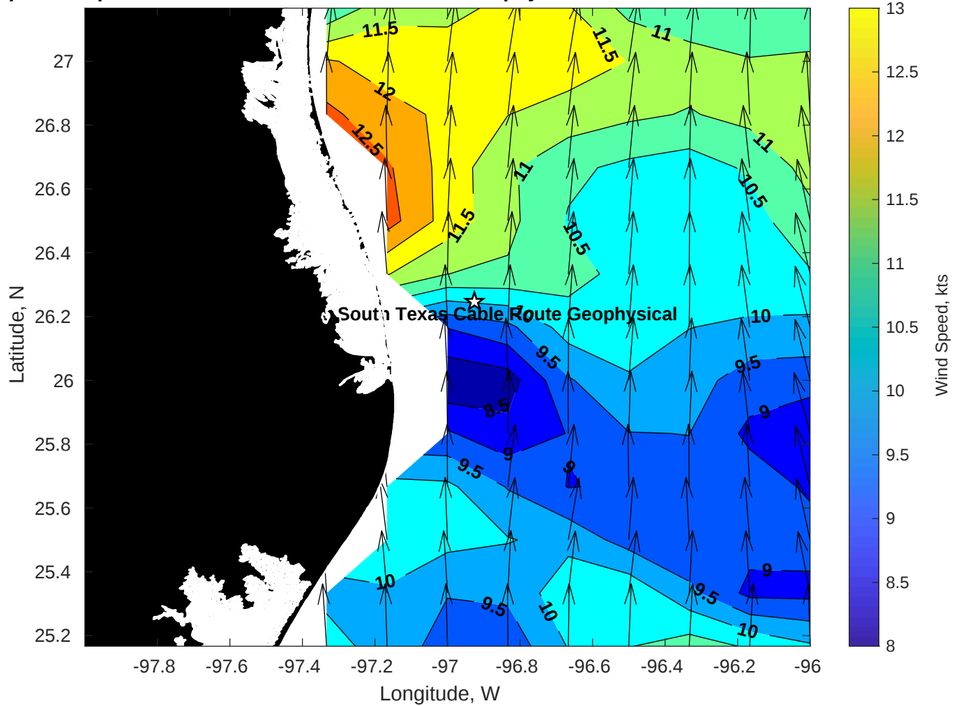
Winds (kts) for Tampnet P2378 South Texas Cable Route Geophysical at 18-Jul-2025 09:00:00
