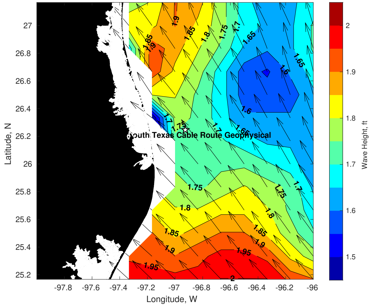
Wave Height (ft) for Tampnet P2378 South Texas Cable Route Geophysical at 18-Jul-2025 09:00:00
