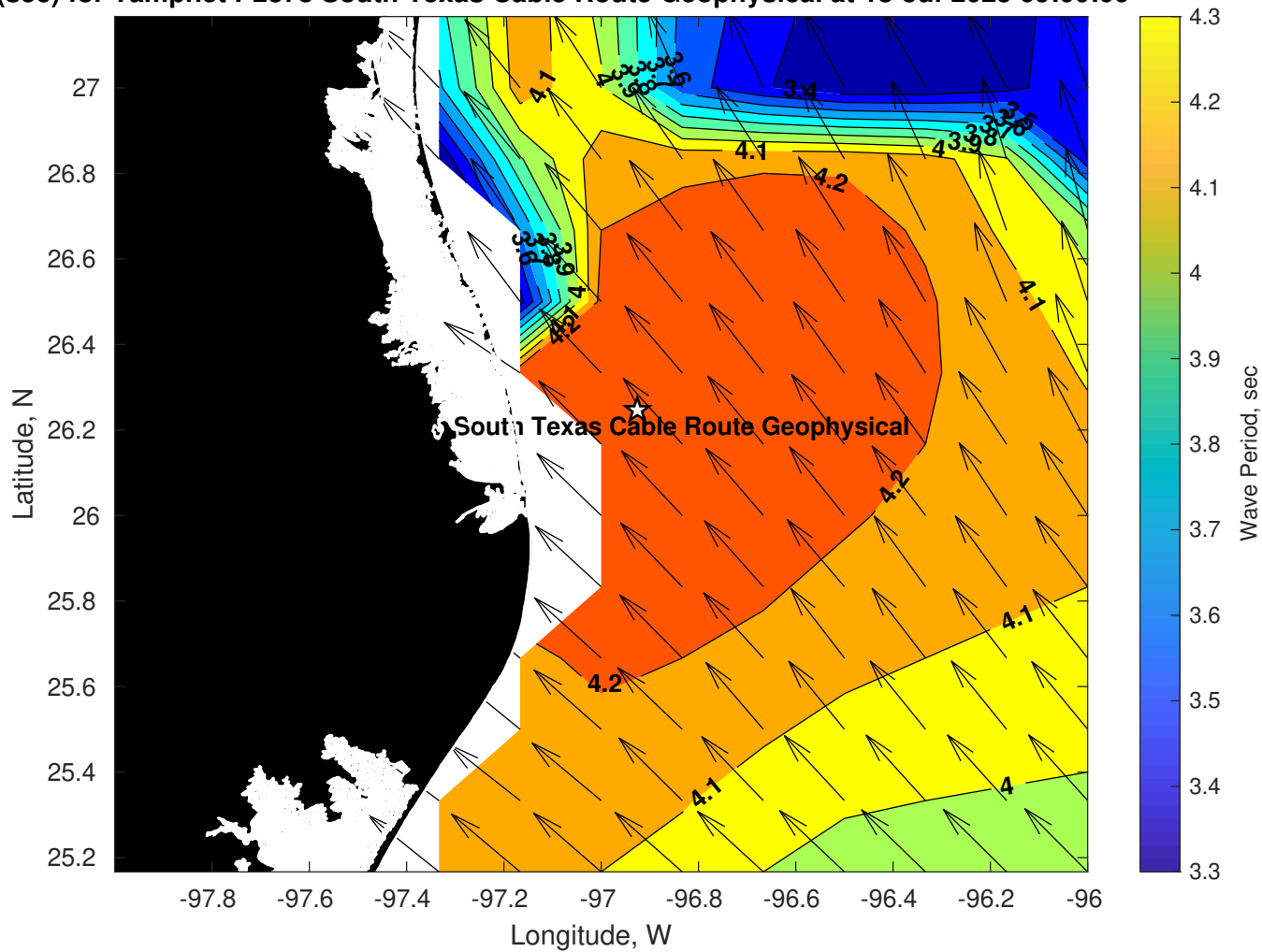
Wave Period (sec) for Tampnet P2378 South Texas Cable Route Geophysical at 18-Jul-2025 09:00:00
