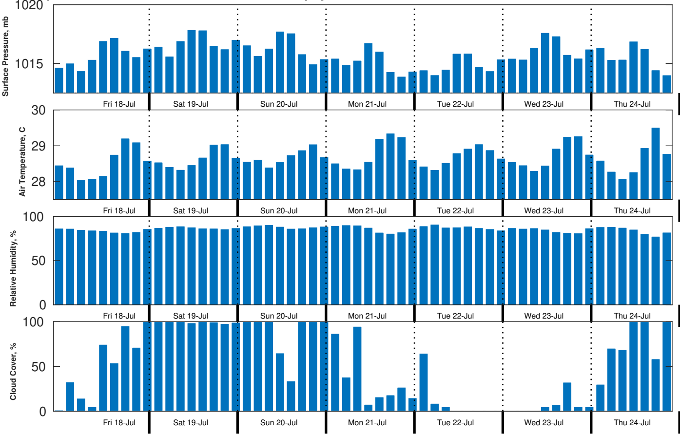
Met Forecast for Tampnet P2378 South Texas Cable Route Geophysical from 18-Jul-2025 00:00:00 to 25-Jul-2025 00:00:00
