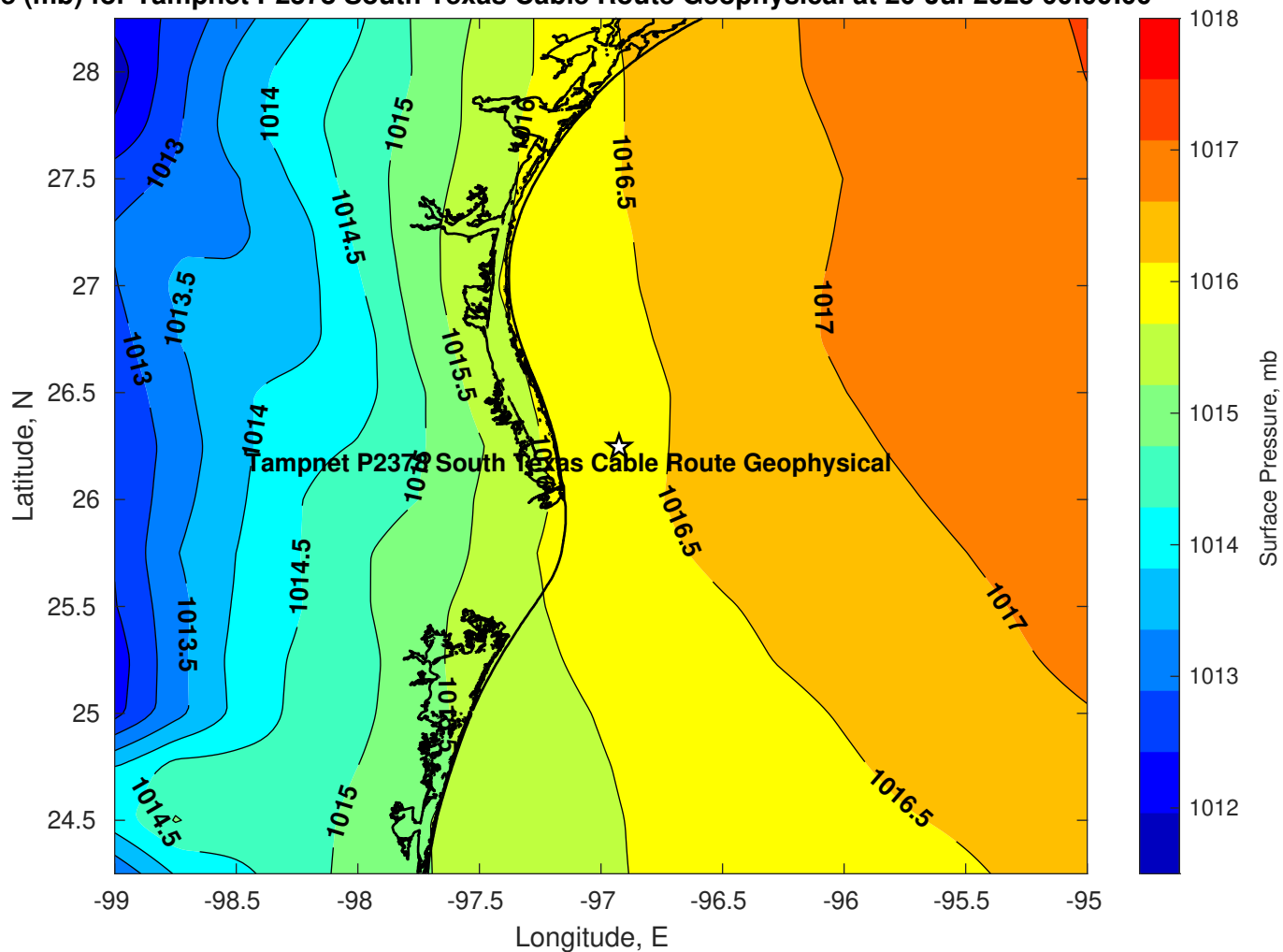
Pressure (mb) for Tampnet P2378 South Texas Cable Route Geophysical at 20-Jul-2025 00:00:00
