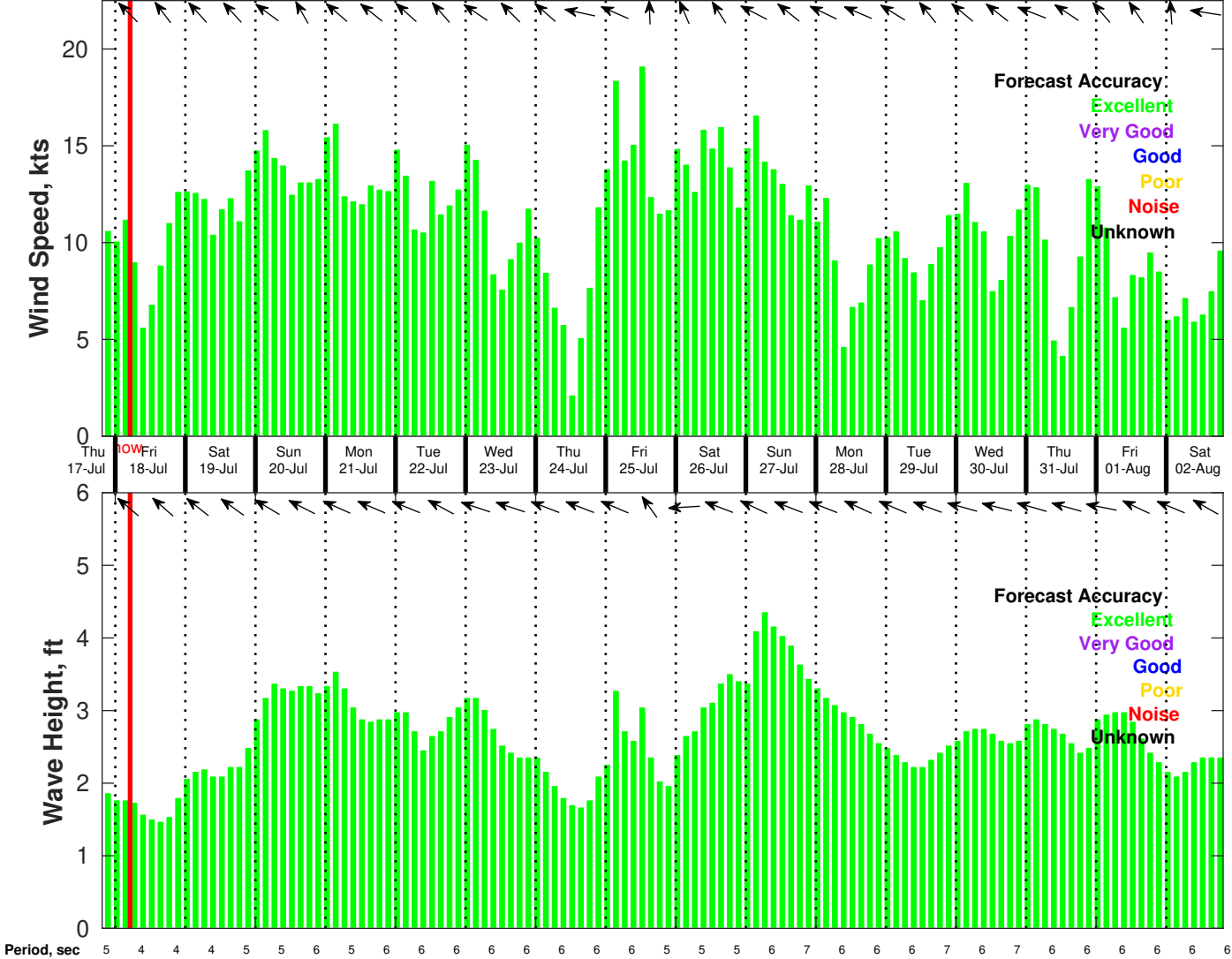
Wind & Wave Forecast for Tampnet P2378 South Texas Cable Route Geophysical from 17-Jul-2025 20:00:00 to 02-Aug-2025 20:00:00
