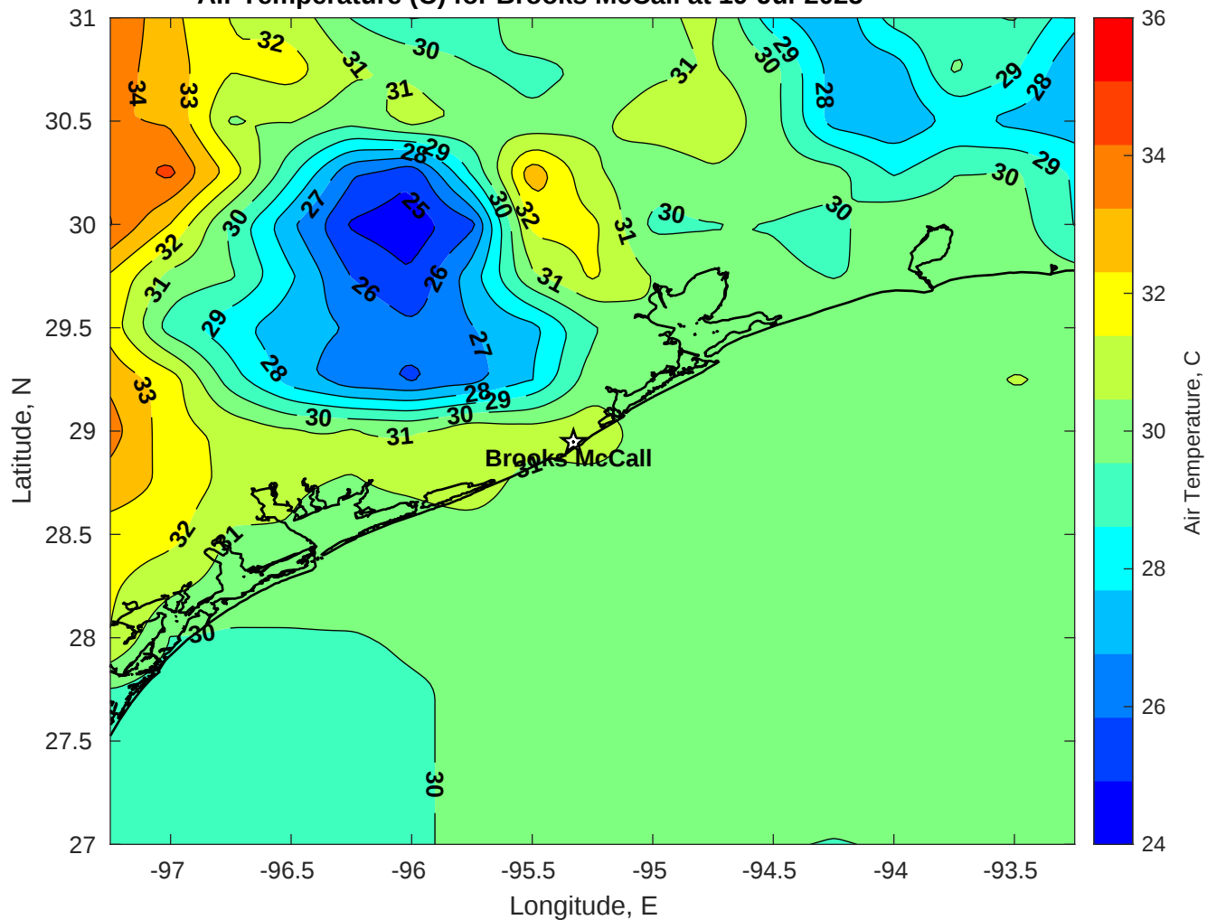
Air Temperature (C) for Brooks McCall at 19-Jul-2025
