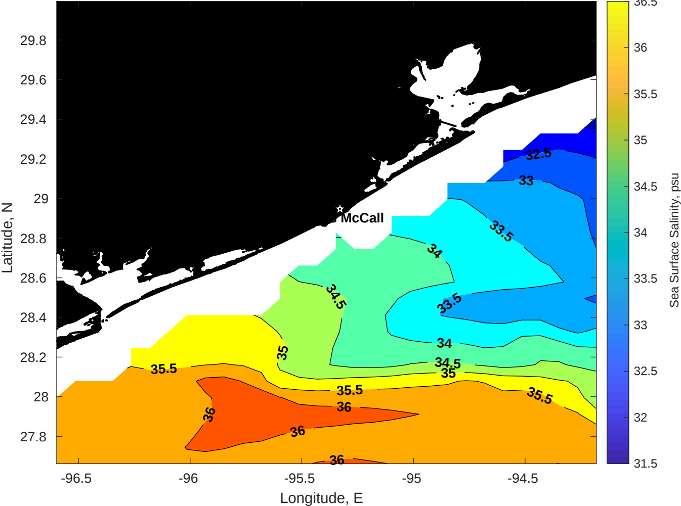
Surface Salinity for Brooks McCall at 18-Jul-2025 00:00:00
