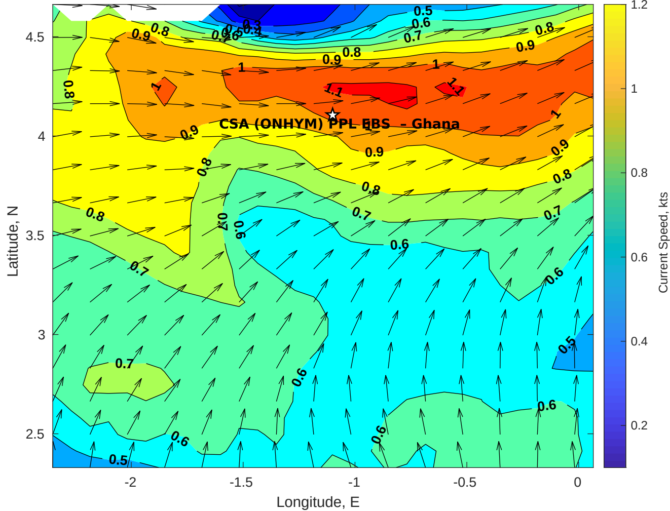
Surface Currents for CSA (ONHYM) PPL EBS - Ghana at 18-Jul-2025 00:00:00
