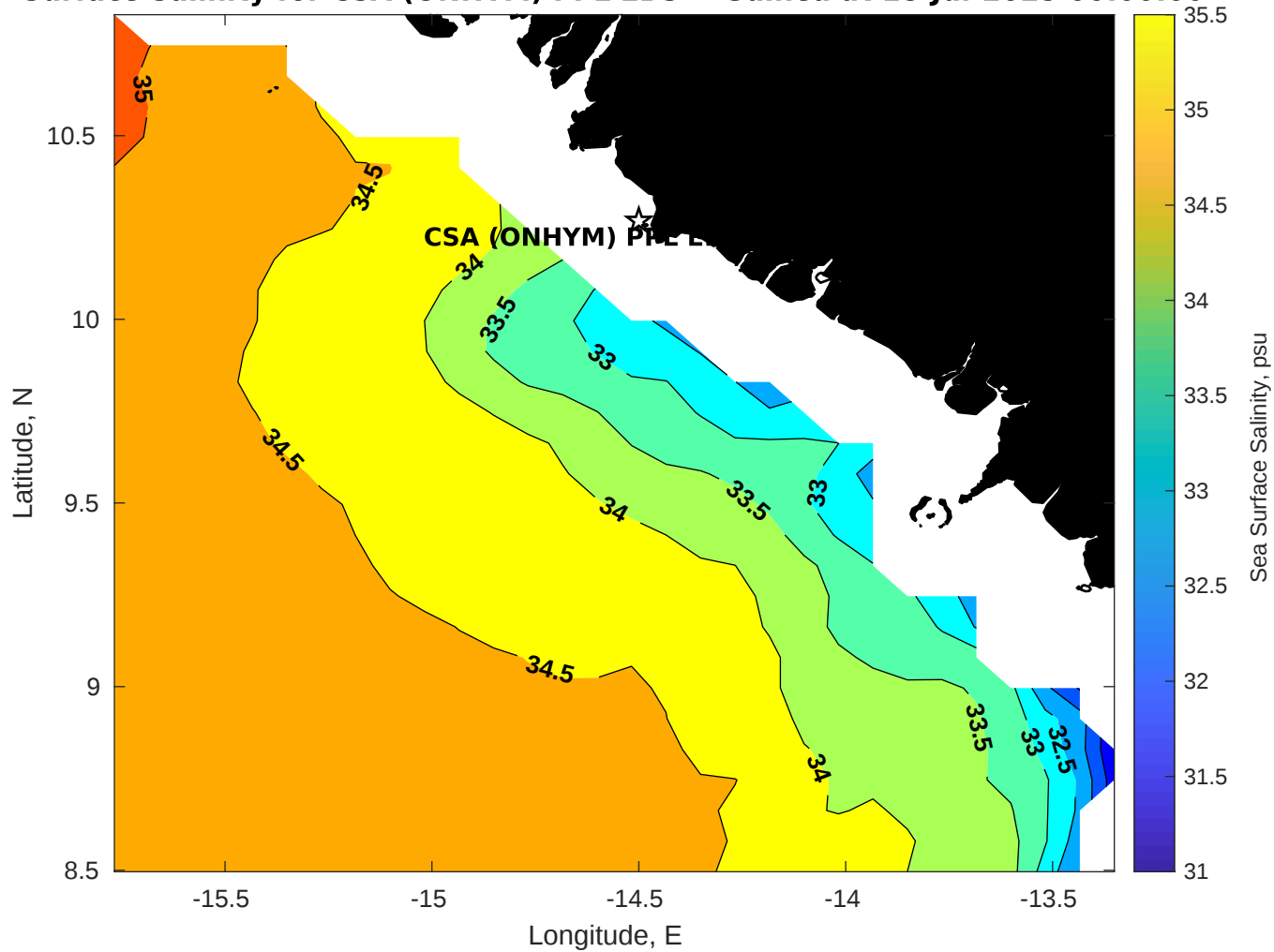
Surface Salinity for CSA (ONHYM) PPL EBS - Guinea at 18-Jul-2025 00:00:00
